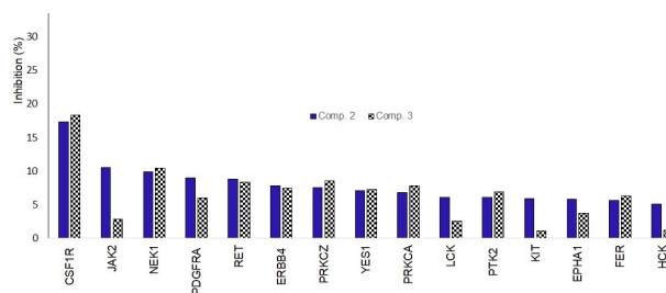
Figure 4. Evaluation of compound 2 and 3 towards a panel of kinases.
