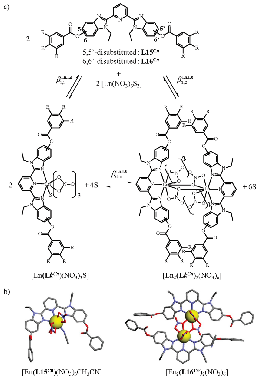
Figure 5. (a) Thermodynamic equilibria for the complexation of L15 Cn or L16 Cn with \text{Ln}(\text{NO}_3)_3 [ \text{R} = \text{H} ( Lk C0 ), \text{OCH}_3 ( Lk C1 ), and \text{OC}_{12}\text{H}_{25} ( Lk C12 ); \text{S} = solvent molecule] and (b) molecular structures of the monomeric [\text{Eu}(\text{L15}^{\text{C0}})(\text{NO}_3)_3\text{CH}_3\text{CN}] and dimeric [\text{Eu}_2(\text{L16}^{\text{C0}})_2(\text{NO}_3)_6] complexes determined by X-ray diffraction. 15
