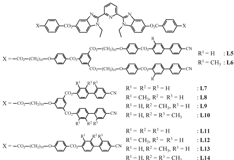
Figure 3. Chemical structures of the symmetrical ligands L5–L14 considered in this contribution.
