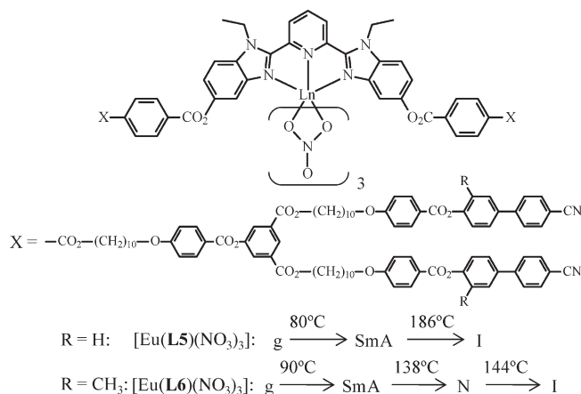
Figure 2. Chemical structures and mesogenic behaviors of the symmetrical dendrimeric complexes [\text{Ln}(\text{Lk})(\text{NO}_3)_3] ( Lk = L5 and L6 ). The phase sequences and transition temperatures are given for Ln = Eu as a typical example (g = glass, SmA = smectic A, N = nematic, and I = isotropic liquid). 10b
