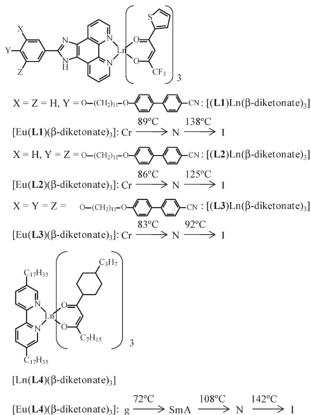
Figure 1. Chemical structures of the nematogenic complexes [\text{Ln}(\text{Lk})(\beta\text{-diketonate})_3] ( Lk = L1–L4 ). The phase sequences and transition temperatures are given for Ln = Eu as a typical example (g = glass, Cr = crystal, SmA = smectic A, N = nematic, and I = isotropic liquid). 8
