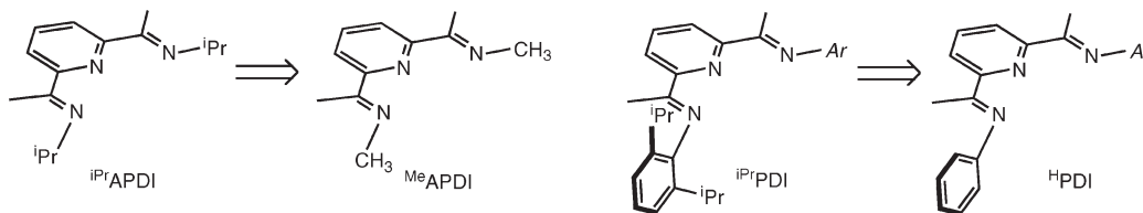
Figure 10. Truncated versions of the bis(imino)pyridine ligands used for DFT studies to examine the origin of the observed distortion in ( iPr APDI)CoCl compounds.
