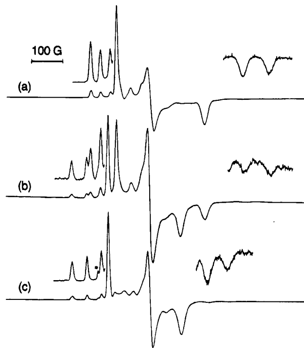
Figure 8. EPR spectra at 77 K generated by the reaction of L a MoO 2 -Cl and a 7-fold excess of Bu n 4 NSH in THF/MeCN (10/1): (a) frozen within 4 min and recorded; (b) frozen after 2.5 h and recorded; (c) frozen after 10 h and recorded. Asterisk: signal from Bu n 4 NSH solution.
