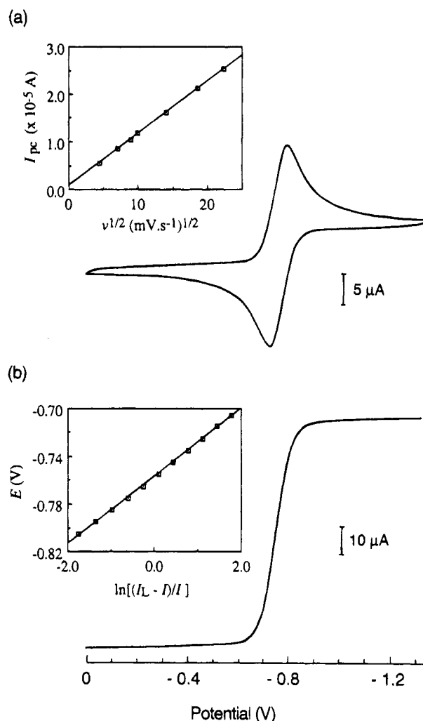
Figure 4. (a) Cyclic voltammogram of L^a\text{MoO}_2(\text{SPh}) (0.5 mM) in MeCN ( \nu = 100 \text{ mV s}^{-1} ; 0.2 M \text{Bu}_4\text{NBF}_4 ). Inset: plot of I_{pc} versus \nu^{1/2} . (b) Rotating disk voltammogram of the same solution ( \nu = 50 \text{ mV s}^{-1} ; \omega = 262 \text{ s}^{-1} ). Inset: plot of E versus \ln[(I_L - I)/I] .
