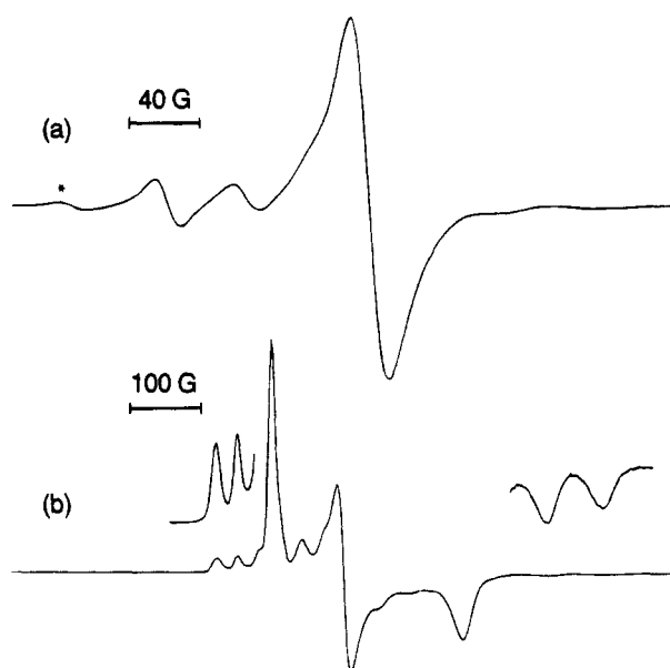
Figure 7. EPR spectra generated by the reaction of \text{L}^a\text{MoO}_2(\text{SPh}) and a 7-fold excess of \text{Bu}_4\text{NSH} in \text{THF}/\text{MeCN} (10/1), recorded after 5 h: (a) 293 K; (b) 77 K. Asterisk: signal from \text{Bu}_4\text{NSH} solution.
