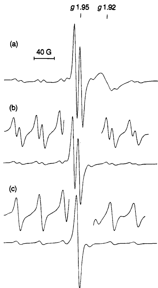
Figure 5. EPR spectra generated by electrochemical reduction of L a -MoO 2 (SPh) at 293 K: (a) 0.2 M Bu 4 NBF 4 in THF dried over activated alumina (the broad feature is due to [L a MoO 2 (SPh)] - ); (b) 1 M 1 H 2 O and 0.2 M Bu 4 NBF 4 in THF; (c) 1 M 2 H 2 O and 0.2 M Bu 4 NBF 4 in THF.
