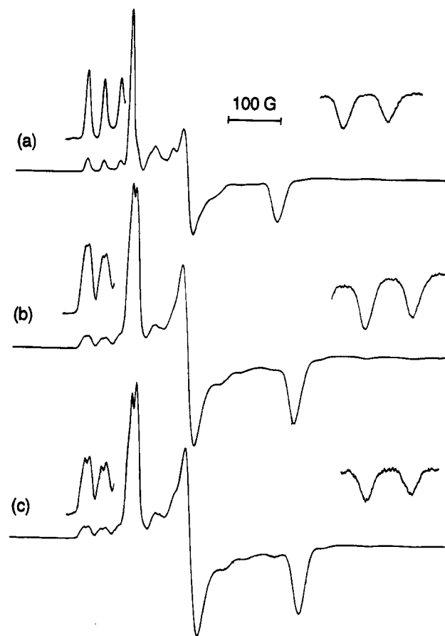
Figure 9. EPR spectra at 77 K generated by the reduction of LMoO 2 -Cl by a 7-fold excess of Bu n 4 NSH in THF/MeCN (10/1), showing 35,37 Cl coupling in one direction: (a) L a ; (b) L b ; (c) L c .
