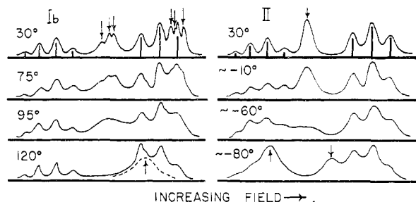
Fig. 1.—Nuclear magnetic resonance spectra of protons of 1-ethylaziridine (Ib) and 1-ethyl-2-methyleneaziridine (II) as a function of temperature. Heavy vertical lines mark characteristic resonance lines of the ethyl group while vertical arrows indicate absorption of the ring hydrogens. The temperature-invariant absorption of the double-bond methylene protons of II is off scale on the left.
