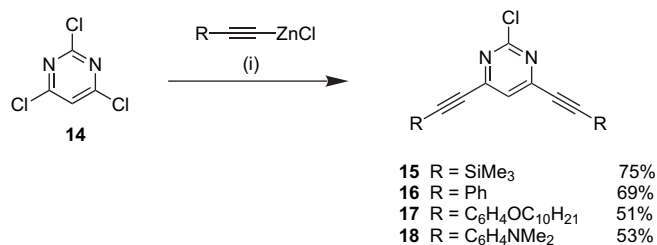
Scheme 4. (i) \text{Pd}(\text{PPh}_3)_4 , THF, 30 °C, 3 h.
