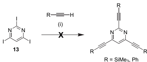
Scheme 3. (i) \text{PdCl}_2(\text{PPh}_3)_2/\text{CuI} , THF/ \text{NEt}_3 , rt, 15 h.
