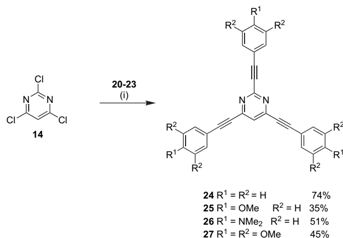
Scheme 7. (i) \text{PdCl}_2(\text{dppf}) \cdot \text{CH}_2\text{Cl}_2/\text{Cs}_2\text{CO}_3 , THF/ \text{H}_2\text{O} , \Delta , 12 h.
