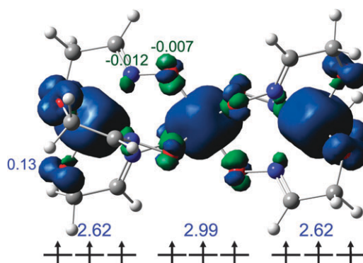
Fig. 2 Spin density distribution for the simplified complex 1 ( \text{R} = \text{H} , not Ph) for clarity. NPA-derived atomic spin densities are shown for Mn, N, and O atoms.
