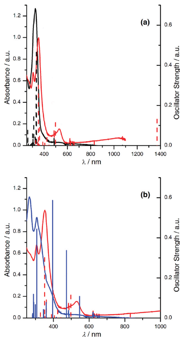
Figure 9. UV-vis-NIR spectroelectrochemistry of qLu-TP. Superimposed experimental plots (black, [qLu-TP] 2+ native; red, [qLu-TP] + singly reduced; blue, [qLu-TP] 0 doubly reduced) and corresponding calculated electronic transitions: pyramidal (solid vertical lines) and axial (dashed vertical lines). (a) [qLu-TP] 2+ and [qLu-TP] + . 38 (b) [qLu-TP] + and [qLu-TP] 0 .
