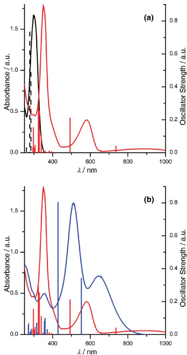
Figure 7. UV–vis–NIR spectroelectrochemistry of Me- TP . Superimposed experimental plots (black, [Me- TP ] + native; red, [Me- TP ] 0 singly reduced; blue, [Me- TP ] − doubly reduced) and corresponding calculated electronic transitions: pyramidal (solid vertical lines) and axial (dashed vertical lines). (a) [Me- TP ] + and [Me- TP ] 0 . (b) [Me- TP ] 0 and [Me- TP ] − . Note that no energy minimum was found for reduced axial forms (see Table S4).
