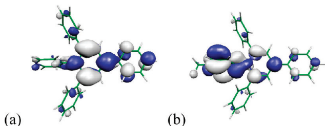
Figure 11. Switching of the site of first reduction upon quaternization. (a) LUMO of Py-TP (the pyridinium core is reduced first). (b) LUMO of qPy-TP (the pendant pyridylum is reduced first); isocontour = 0.025.
