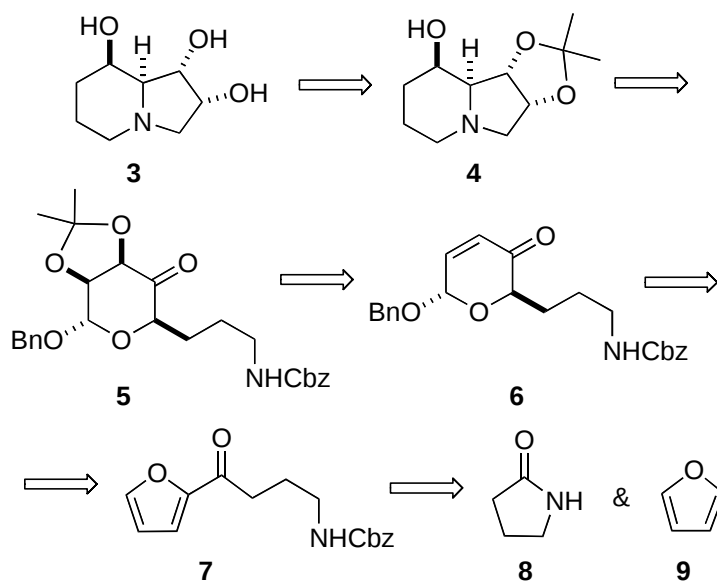
Scheme 1. Retrosynetical analysis
