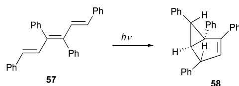
Scheme 13 Photochemical transformation of triene 57 .
