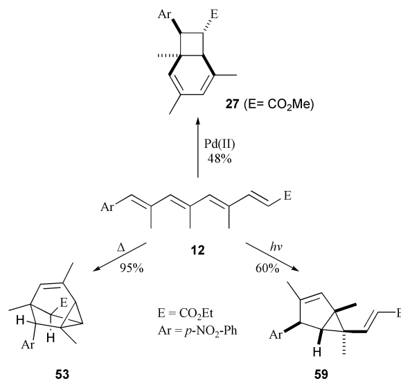
Scheme 18 Cascade electrocyclic pathways of tetraene ester 12 .
