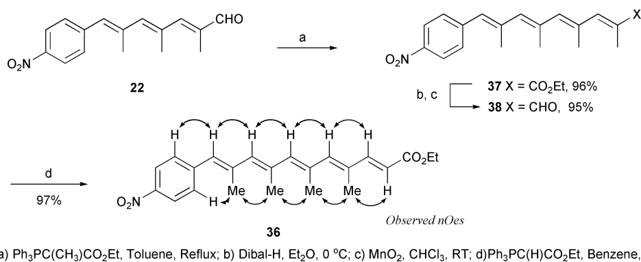
Scheme 7 Synthesis of pentaene 36 .
