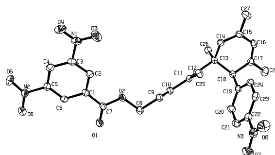
Fig. 4 X-Ray structure of 41 .
