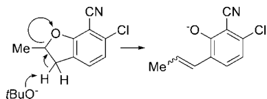
Figure 4. Base-promoted opening reaction of dihydrobenzofuran 33 .
