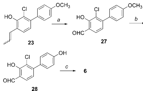
Scheme 3. Synthesis of 3-Chloro-Substituted Salicylaldoxime 6 a
