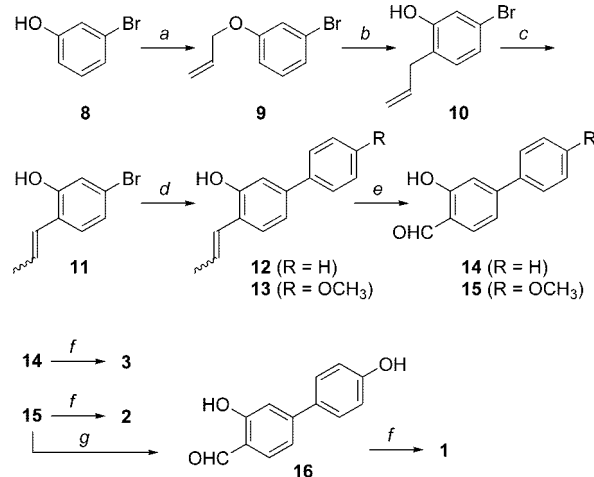
Scheme 1. Synthesis of 3-Unsubstituted Salicylaldoximes 1–3 a
