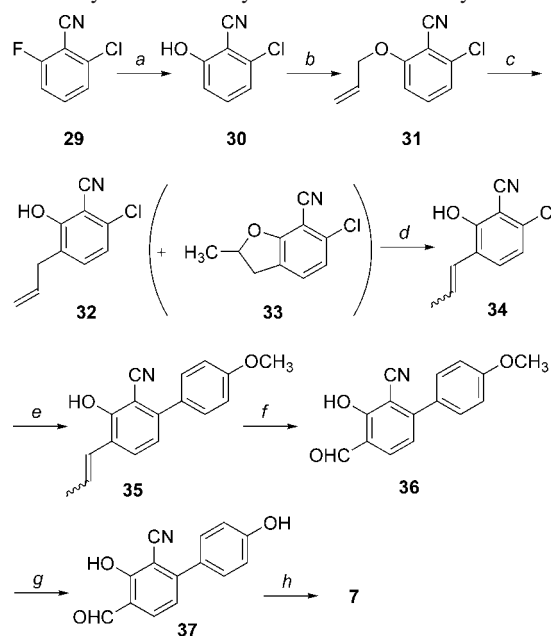
Scheme 4. Synthesis of 3-Cyano-Substituted Salicylaldoxime 7 a
