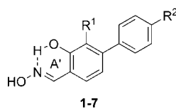
Chart 1. Monoaryl-Substituted Salicylaldoximes Designed as ER \beta -Selective Ligands
