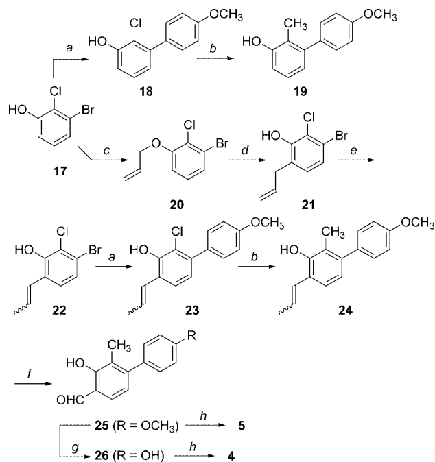
Scheme 2. Synthesis of 3-Methyl-Substituted Salicylaldoximes 4 and 5 a
