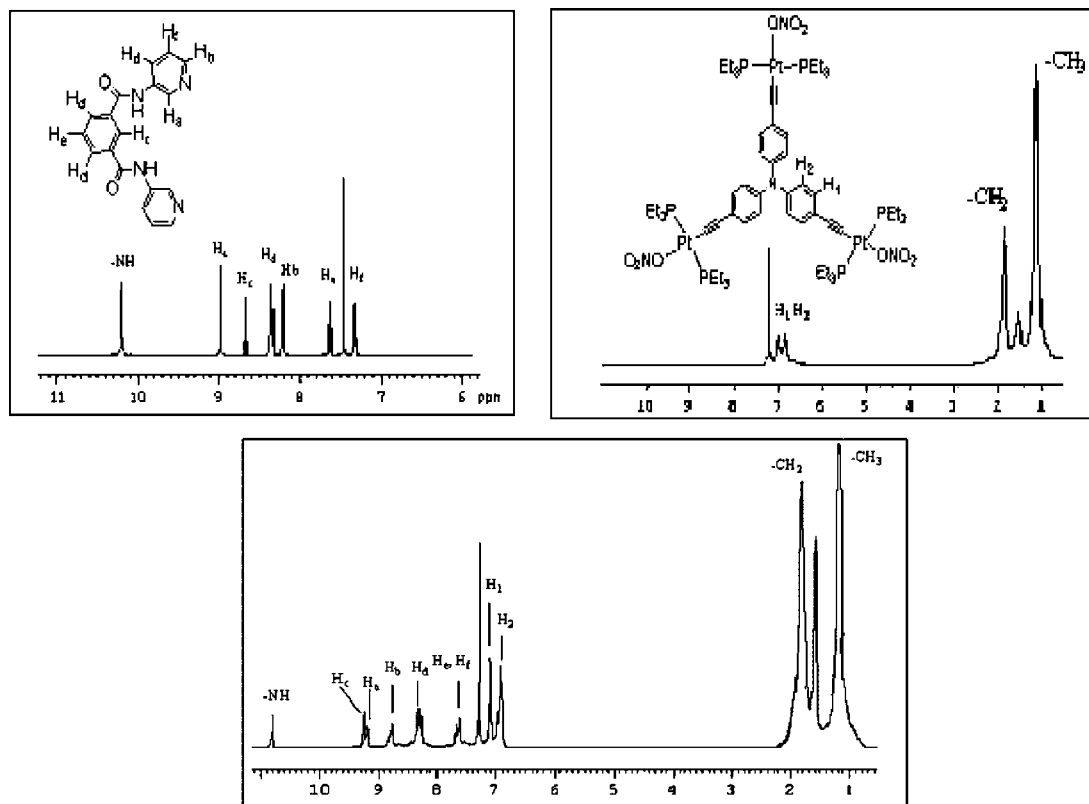
Figure 2. ^1\text{H} NMR of L (top left), M (top right), and 1 (bottom) in \text{CDCl}_3 .
