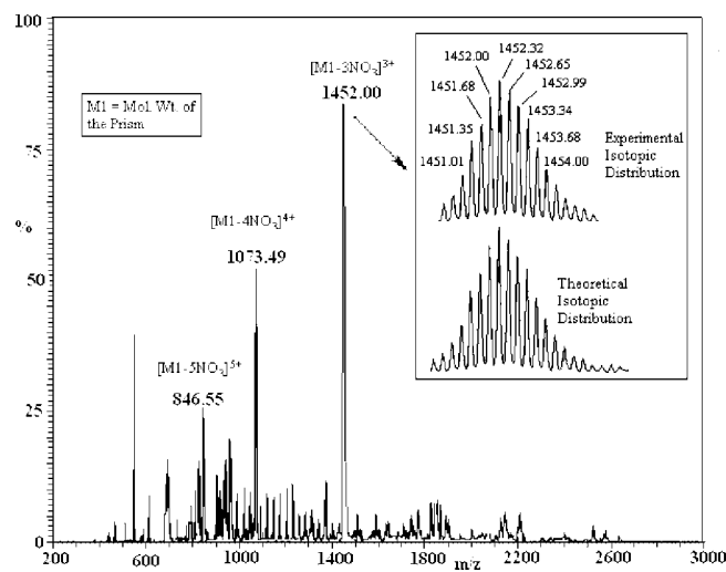
Figure 3. ESI-MS spectrum of 1 in MeOH. Inset: theoretical and experimental isotopic distribution patterns of the [\text{M1-3NO}_3]^{3+} peak.
