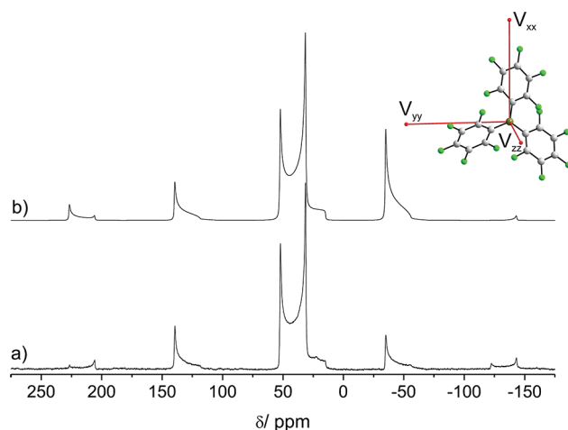
Figure 4. ^{11}\text{B} MAS NMR spectrum of the educt of the 1,1-carbaboration, \text{B}(\text{C}_6\text{F}_5)_3 ( 12 ), acquired at 11.7 T with a rotation frequency of 14 kHz (a) and simulated spectrum using the SIMPSON program package (b) assuming a C_Q of 4.3 MHz, an \eta value of 0.02, and \Delta\sigma = 300 ppm. The inset on top shows the DFT calculated (B97-D, def2-TZVP (modified), see Experimental Section) orientation of the EFG in the molecular axis frame. V_{zz} is oriented perpendicular to the boron coordination plane.
