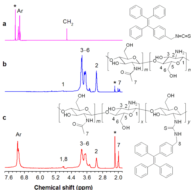
Figure 1. ^1\text{H} NMR spectra of (a) TPE-ITC, (b) CS, and (c) TPE-CS measured in (a) chloroform- d_4 and (b, c) an acetic acid- d_4 /water- d_2 mixture at room temperature. The solvent peaks are marked with asterisks.
