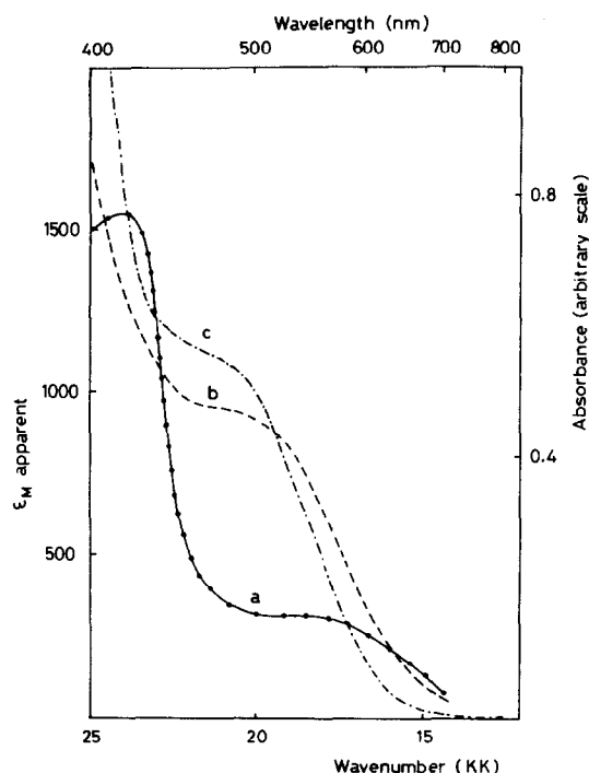
Fig. 1. Electronic absorption spectra: (a) —●—, [\text{Co}(\text{HP}(\text{CH}_3)\text{Ph})_5](\text{H}_2\text{O})(\text{BF}_4)_2 (green form) in Nujol mull; (b) — — —, [\text{Co}(\text{HP}(\text{CH}_3)\text{Ph})_5](\text{BF}_4)_2 (red form) in Nujol mull; (c) — · — · —, [\text{Co}(\text{HP}(\text{CH}_3)\text{Ph})_5](\text{BF}_4)_2 , 2.32 \times 10^{-3} \text{ M} in acetone containing 1.6 \text{ M} methylphenylphosphine.
