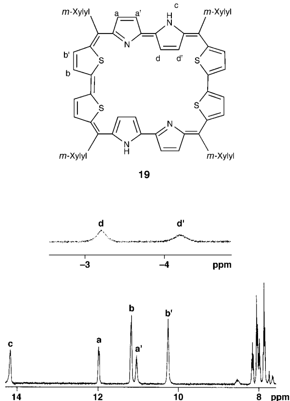
Figure 2. ^1\text{H} NMR spectrum of 19 in \text{CDCl}_3 at 298 K in the low field region. The assignments are marked based on the ^1\text{H} , ^1\text{H} COSY spectrum. The inset shows the up field region.
