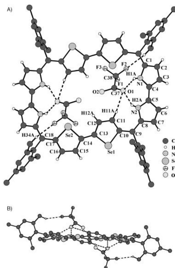
Figure 4. A) Top view of the TFA bound complex of octaphyrin, 14 . B) Side view; the meso -mesityl rings and noninteracting hydrogens which are not involved in the hydrogen bonding are omitted for clarity.
