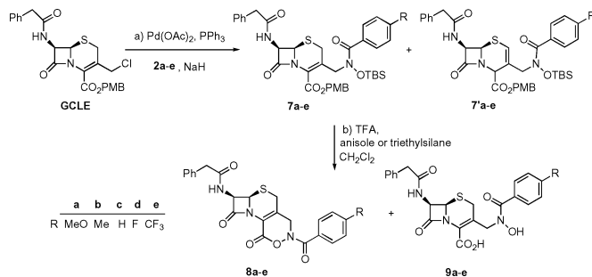
Scheme 3 Synthesis of 8a–e and 9a–e . a) GCLE (1.0 equiv.), \text{Pd}(\text{OAc})_2 (0.12 equiv.), \text{PPh}_3 (0.60 equiv.), 2a–e (1.1 equiv.), NaH (1.0 equiv.), 0 °C–rt, 3 h; b) TFA (14 equiv.), anisole (or triethylsilane) (4.0 equiv.), \text{CH}_2\text{Cl}_2 , 0 °C–rt, 1.5 h.
