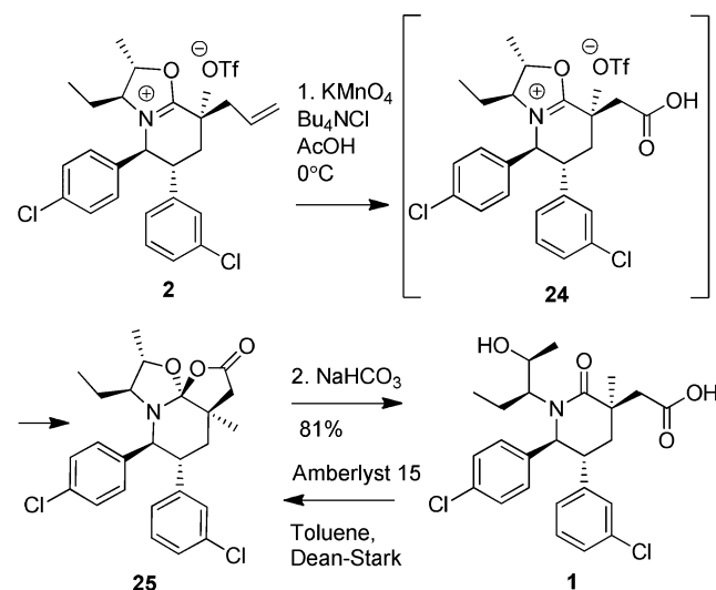
Scheme 6. Bicyclic Iminium Ether 2 As a Hydroxyl Protecting Group and the Synthesis of 1
