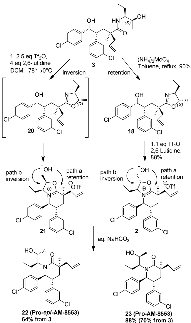
Scheme 5. Oxazoline-Assisted Cyclization Utilizing 2° Hydroxyl Amino Alcohols
