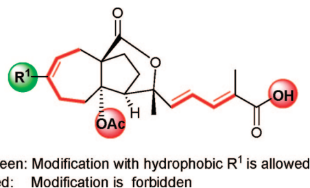
Figure 4. SAR of pseudolaric acid B analogs.
