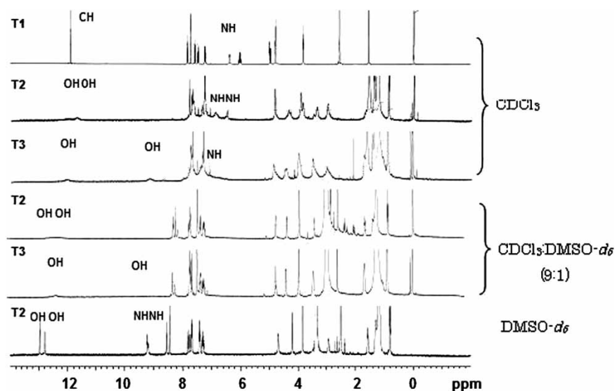
Figure 2. 1 H NMR spectrum of T1 – T3 in CDCl 3 and T2 , T3 in CDCl 3 :DMSO- d 6 (9:1); T2 in DMSO- d 6 .
