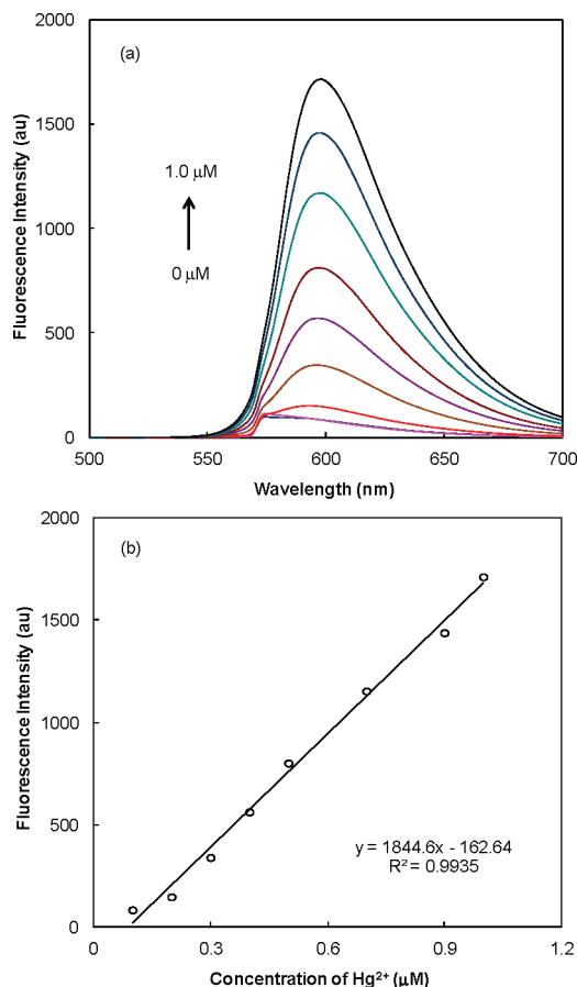
Figure 2. (a) Fluorescence titration spectra ( \lambda_{\text{ex}} = 570 nm, with slit widths of 2.5 nm) of probe 1 (20 \mu\text{M} in pure water) with \text{Hg}^{2+} from 0 to 1.0 \mu\text{M} at room temperature (reacted 15 min and adjusted pH to 7.4 with PBS before determination). (b) The plot of fluorescence intensity changes ( \lambda_{\text{ex}}/\lambda_{\text{em}} = 570/594 nm, slit widths of 2.5 nm) of probe 1 (20 \mu\text{M} in pure water) against varied concentration of \text{Hg}^{2+} from 0.1 to 1.0 \mu\text{M} at room temperature (reacted 15 min and adjusted pH to 7.4 with PBS before determination).
