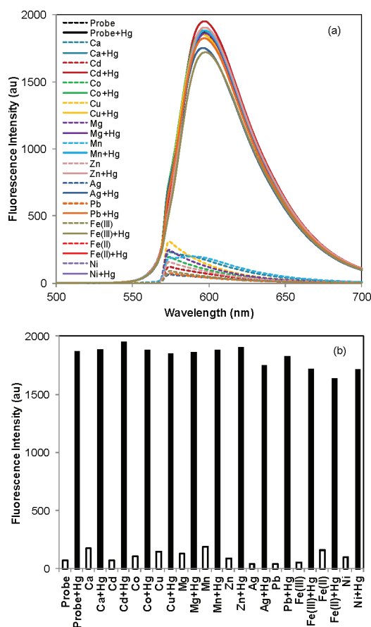
Figure 3. (a) Fluorescence spectra ( \lambda_{\text{ex}} = 570 nm, with slit widths of 2.5 nm) of probe 1 ( 20 \mu\text{M} in pure water) upon addition of various metal ions ( 1.0 mM in pure water). Dot line: probe 1 + metal cation, solid line: probe 1 + metal cation + \text{Hg}^{2+} (reacted 15 min and adjusted pH to 7.4 with PBS before determination). (b) Fluorescence response ( \lambda_{\text{ex}}/\lambda_{\text{em}} = 570/594 nm, with slit widths of 2.5 nm) of probe 1 ( 20 \mu\text{M} in pure water) upon addition of various metal cations ( 1.0 mM in pure water). White column: probe 1 + metal cation, black column: probe 1 + metal cation + \text{Hg}^{2+} (reacted 15 min and adjusted pH to 7.4 with PBS before determination).
