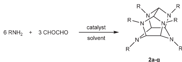
Scheme 1. Condensation of primary amines 1a–g on glyoxal; a : R = 2-thienyl-CH 2 , b : R = PhCH=CH-CH 2 , c : R = 3-pyridyl-CH 2 , d : R = CH 2 =CH-CH 2 , e : R = 2-furfuryl, f : R = CH=CH-CH 2 , g : R = 1-naphthyl-CH 2 , h : R = CH 2 =CH-CHMe, i : R = PhCHMe, j : R = CH 2 =CH-CMe 2 , k : R = PhCMe 2 .
