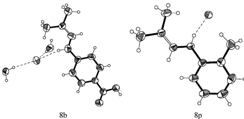
Fig. 1. ORTEP view of crystal structures of 8b and 8p with 35% probability ellipsoids.
