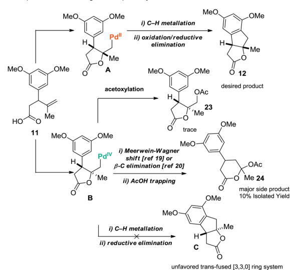
Figure 4. Proposed mechanisms for difunctionalization cascade and degradation pathways.
