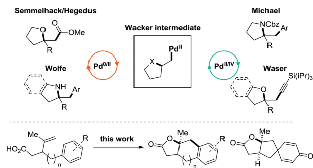
Figure 1. Pd-mediated oxidative C–C bond forming cyclizations.
