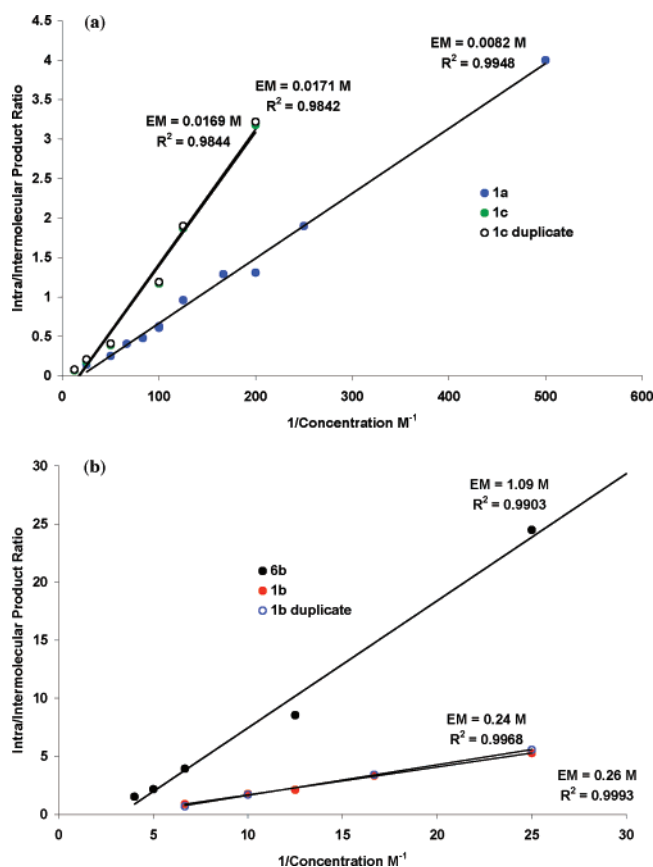
FIGURE 4. Determination of effective molarities for the RCMs of (a) 1a and 1c and (b) 1b and 6b (DCM, 5 mol % 3 , 30 mol % Ti(O- i Pr) 4 , reflux, 18 h).
