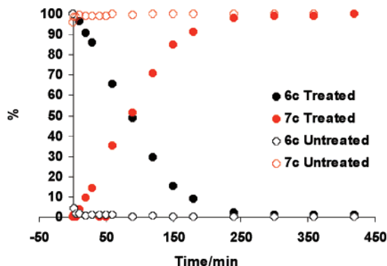
FIGURE 1. Substrate consumption appears instantaneously in the absence of sample treatment. RCM of 6c (0.01 M in DCM, 1 mol % 3 , 30 mol % Ti(O- i Pr) 4 , 25 ± 0.1 °C).
