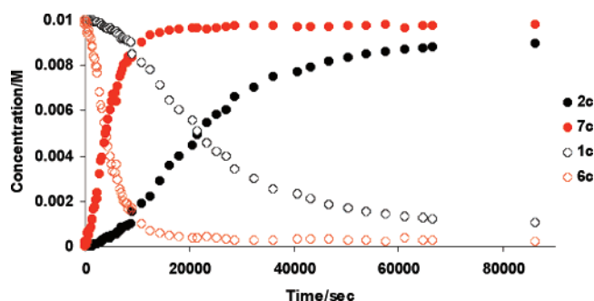
FIGURE 3. Competitive RCM between gem -dimethylated 6c and less substituted 1c (0.01 M in each substrate in DCM, 2 mol % 3 , 30 mol % \text{Ti}(\text{O}-i\text{Pr})_4 per substrate, 25 \pm 0.1 °C, treated aliquots).
