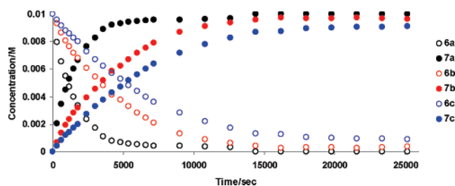
FIGURE 2. Competitive RCM between substrates 6a , 6b , and 6c (0.01 M in each substrate in DCM, 2 mol % 3 , 30 mol % \text{Ti}(\text{O}-i\text{Pr})_4 per substrate, 25 \pm 0.1 °C, treated aliquots).
