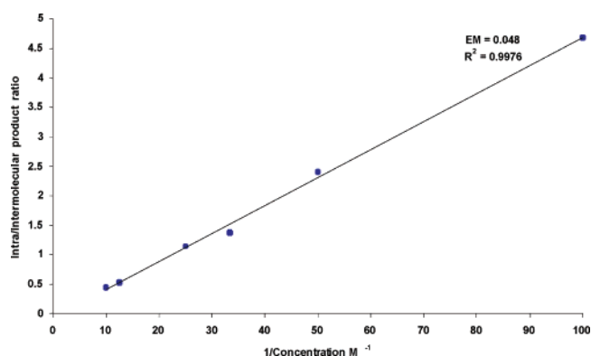
FIGURE 5. Determination of effective molarities for the RCMs of 1b in the absence of the Ti(IV) cocatalyst (DCM, 5 mol % 3 , reflux, 18 h).
