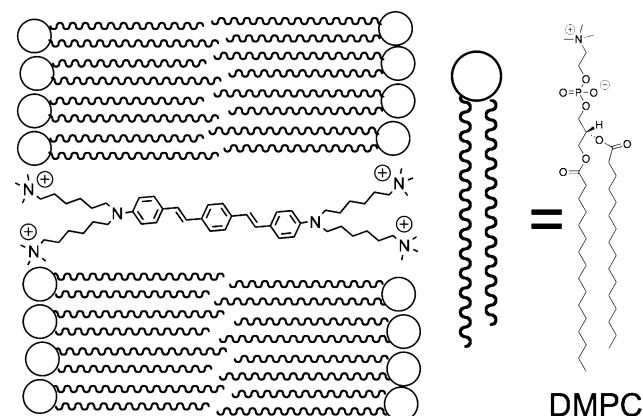
Figure 1. Cartoon representation of a DSBN+ modified lipid bilayer depicting the predicted orientation when intercalated within a phospholipid bilayer. The long molecular axis is normal to the plane of the membrane with the hydrophobic conjugated region within the nonpolar inner membrane and the polar pendant group terminals oriented outward toward the polar aqueous environment on either side of the lipid bilayer.
