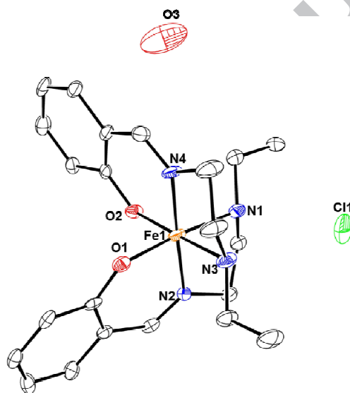
Fig. 1. ORTEP-3 diagram of 1·0.5H 2 O with co-crystallised H 2 O, using 30 % probability level ellipsoids. Hydrogen atoms are omitted for clarity.
