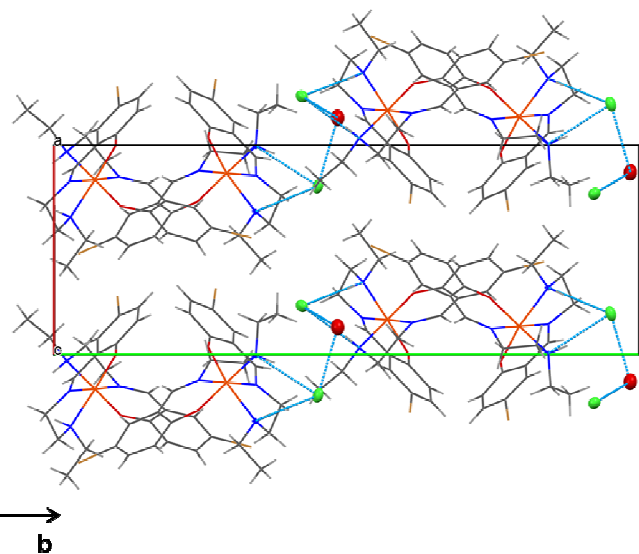
Fig. 4. Mercury packing diagram of 2·0.5H 2 O viewed along the c axis, showing the layers of [Fe(salEen) 2 ] + cations alternating with Cl − anions and H 2 O molecules. Hydrogen bonds between the amine groups of the salEen cations and the Cl − anions are represented as light blue dashed lines.
