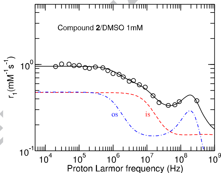
Fig. 7. Fit of the r_1 dispersion for 1 mM of compound 2 using Eqs. (2) and (3). The contributions of the is (dashed) and os (dash dot) to the total r_1 are also shown.
