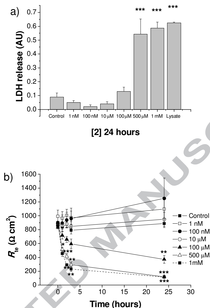
Fig. 8. High concentrations of compound 2 exert toxic effects on T84 monolayers. a) T 84 monolayers were treated bilaterally with compound 2 for 24 hours. An equal aliquot of apical and basolateral medium was used to measure LDH release from the cells ( n = 4 - 8 ). b) T 84 monolayers were treated with compound 2 at various concentrations (1 nM to 1 mM) over a 24 hr period during with R_{te} was measured ( n = 4 - 8 ).
