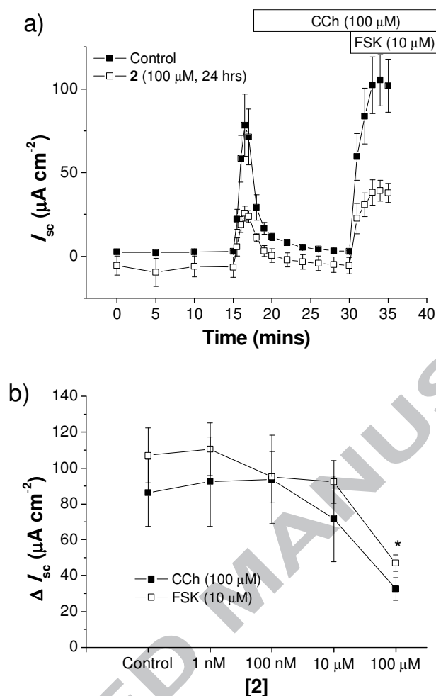
Fig. 9. Compound 2 attenuates Cl - secretion across T 84 cells. a) T 84 cell monolayers were treated bilaterally with compound 2 (100 \mu M ) in serum-free medium for 24 hrs. Cells were then washed and mounted in Ussing chambers, and I_{sc} responses to CCh (100 \mu M ) and FSK (10 \mu M ) were measured ( n = 6 - 8 ). b) T 84 monolayers were treated with compound 2 at various concentrations (1 nM to 100 \mu M ) for 24 hrs before I_{sc} responses to CCh and FSK were measured ( n = 6 - 8 ).
