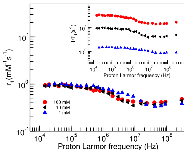
Fig. 5. r_1 dependence with \nu_{L,H} at concentrations 1, 10 and 100 mM for compound 2 . The inset shows the relaxation rate for the same samples.
