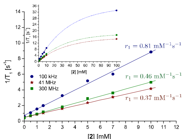
Fig. 6. 1/T_1 vs [2] at three different \nu_{LH} (100 kHz, 41 MHz and 300 MHz) and the corresponding r_1 values. The inset plot also shows the values of 1/T_1 for 100 mM where a clear deviation from the linear behaviour is observed. The dotted lines are a guide for the eyes.
