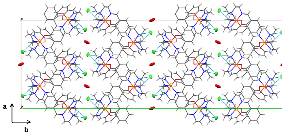
Fig. 2. Mercury packing diagram of 1·0.5H 2 O viewed along the c axis showing the layers of [Fe(salEen) 2 ] + cations alternating with Cl − anions and H 2 O molecules. Hydrogen bonds between the amine groups of the salEen cations and the Cl − anions are represented as light blue dashed lines.
