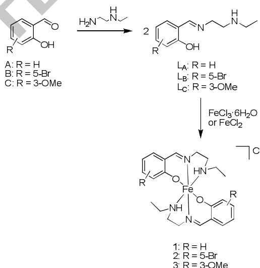
Scheme 1. General method used in the synthesis of complexes 1-3 .
