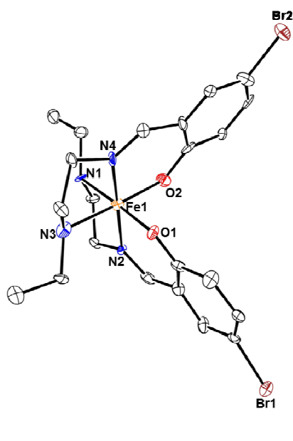
Fig. 3. ORTEP-3 diagram of 2·0.5H 2 O ( molecule 1 ) with co-crystallised H 2 O, using 30 % probability level ellipsoids. Hydrogen atoms are omitted for clarity.
