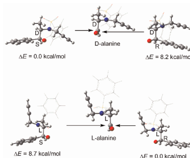
Figure 2. Grignard reagent attack on carbonyl group of D and L forms of alanine derivatives. For clarity, the tosyl group substituent is represented in wireframe.
