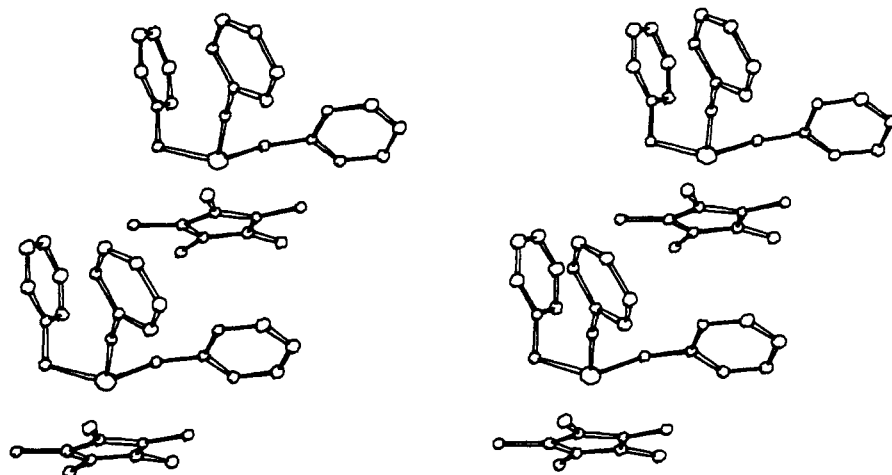
Figure 3. Stereopair showing snug fit between molecules. The orientation is the same as in Figure 2. The Cp ring of one molecule is situated between the three "Phenyl-legs" of the molecule translated by b .
