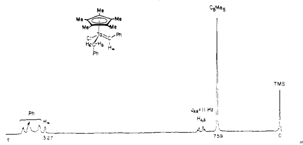
Figure 1. 270-MHz 1 H NMR spectrum of Ta(η 5 -C 5 Me 5 )(CHPh)(CH 2 Ph)Cl in C 6 D 6 .
