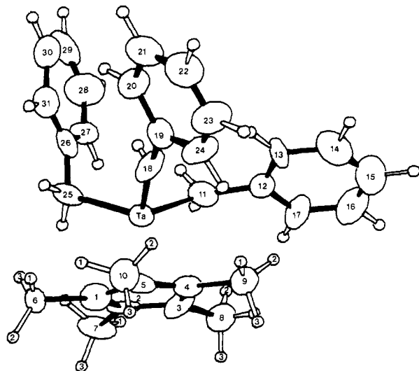
Figure 2. A computer drawing of \text{Ta}(\eta^5\text{-C}_5\text{Me}_5)(\text{CHPh})(\text{CH}_2\text{Ph})_2 . Carbon atoms are numbered as in Table II. Hydrogen atoms are referred to by the numbers of the associated carbon atoms. Methyl hydrogen atoms are further distinguished by numbers 1-3.
