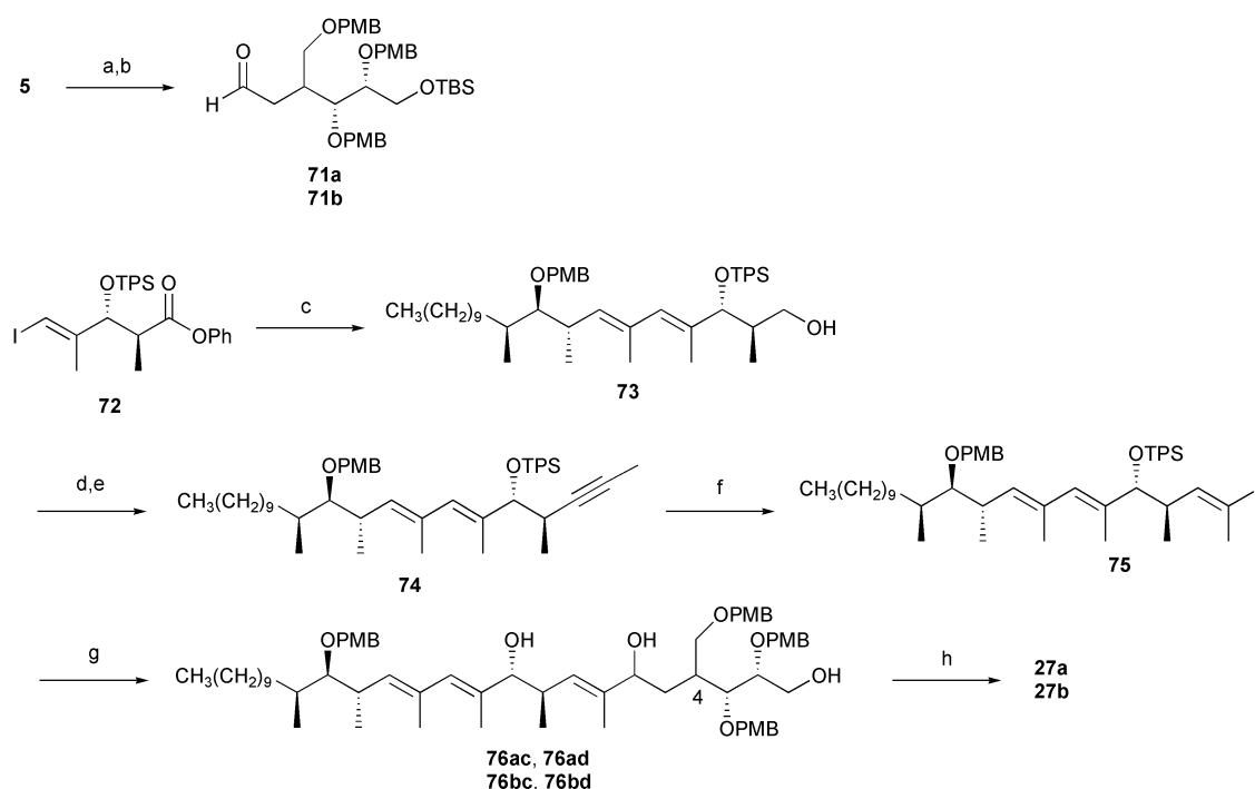
Scheme 12 Synthesis of 27 . Reagents and conditions: (a) i) (\text{COCl})_2 , DMSO, \text{Et}_3\text{N} , \text{CH}_2\text{Cl}_2 , ii) \text{PPh}_3=\text{CHCO}_2\text{Et} , THF, reflux, iii) \text{NiCl}_2 , \text{NaBH}_4 , THF, EtOH, 3 steps, 77%; (b) DIBAL, \text{CH}_2\text{Cl}_2 , 36% ( 71a ), 57% ( 71b ); (c) i) 3, 9-BBN, THF then \text{PdCl}_2(\text{dppf}) , \text{K}_3\text{PO}_4 , DMF, \text{H}_2\text{O} , 65^\circ\text{C} , ii) DIBAL, \text{CH}_2\text{Cl}_2 , -78^\circ\text{C} , 2 steps, 78%; (d) i) (\text{COCl})_2 , DMSO, \text{Et}_3\text{N} , \text{CH}_2\text{Cl}_2 , ii) \text{PPh}_3 , \text{CBr}_4 , \text{CH}_2\text{Cl}_2 , 2 steps, 92%; (e) n\text{-BuLi} , THF, -78^\circ\text{C} , \text{CH}_3\text{I} , rt, 91%; (f) \text{Cp}_2\text{ZrHCl} , THF then \text{I}_2 , 80%; (g) i) 71a or 71b , \text{NiCl}_2 , \text{CrCl}_3 , DMSO, ii) \text{HCl} , THF, 2 steps, 13% ( 76ac ), 20% ( 76ad ), 15% ( 76bc ), 10% ( 76bd ); (h) i) (\text{COCl})_2 , DMSO, \text{Et}_3\text{N} , \text{CH}_2\text{Cl}_2 , ii) \text{NaClO}_2 , \text{NaH}_2\text{PO}_4 , t\text{-BuOH} , \text{H}_2\text{O} , iii) \text{BCl}_3 , \text{CH}_2\text{Cl}_2 , -78^\circ\text{C} .
