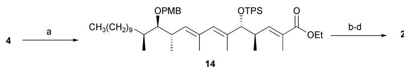
Scheme 4 Synthesis of 2 . Reagents and conditions: (a) 3 , 9-BBN, THF, rt, then PdCl 2 (dppf), K 3 PO 4 , H 2 O, 65 °C, 88%; (b) DIBAL, CH 2 Cl 2 , −78 °C, 94%; (c) i) MnO 2 , CH 2 Cl 2 , ii) NaClO 2 , NaH 2 PO 4 , t -BuOH, H 2 O, 2 steps, 73%; (d) 5 , DCC, DMAP, DMAP·HCl, CH 2 Cl 2 , reflux, 69%.
