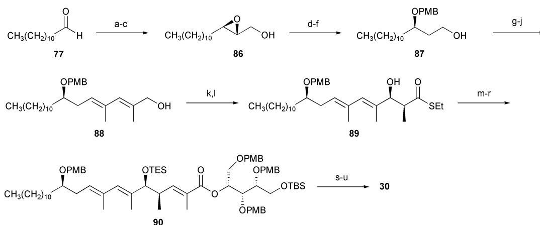
Scheme 14 Synthesis of 30 . Reagents and conditions: (a) \text{Ph}_3\text{P}=\text{CHCO}_2\text{Et} , \text{CH}_2\text{Cl}_2 , 97%; (b) DIBAL, \text{CH}_2\text{Cl}_2 , -78^\circ\text{C} , 88%; (c) \text{Ti}(\text{O}i\text{-Pr})_4 , (D)-DET, TBHP, \text{CH}_2\text{Cl}_2 , -23^\circ\text{C} , 98%; (d) Red-Al, THF, 91%; (e) PMPCH(OMe) _2 , TsOH, \text{CH}_2\text{Cl}_2 , 90%; (f) DIBAL, \text{CH}_2\text{Cl}_2 , -78^\circ\text{C} , 98%; (g) (\text{COCl})_2 , DMSO, \text{Et}_3\text{N} , \text{CH}_2\text{Cl}_2 , 84%; (h) i) \text{Ph}_3\text{P}=\text{C}(\text{CH}_3)\text{CO}_2\text{Et} , THF, ii) DIBAL, \text{CH}_2\text{Cl}_2 , -78^\circ\text{C} , 2 steps, 84%; (i) TPAP, NMO, MS 4A, \text{CH}_2\text{Cl}_2 , 89%; (j) i) \text{Ph}_3\text{P}=\text{C}(\text{CH}_3)\text{CO}_2\text{Et} , THF, ii) DIBAL, \text{CH}_2\text{Cl}_2 , -78^\circ\text{C} , 2 steps, 78%; (k) \text{MnO}_2 , \text{CH}_2\text{Cl}_2 , 95%; (l) chiral \text{Sn}(\text{OTf})_2 -catalyzed aldol reaction (see ref. 3), 78%; (m) TESOTf, 2,6-lutidine, \text{CH}_2\text{Cl}_2 , 85%; (n) DIBAL, \text{CH}_2\text{Cl}_2 , -78^\circ\text{C} , 95%; (o) \text{Ph}_3\text{P}=\text{C}(\text{CH}_3)\text{CO}_2\text{Et} , \text{CH}_2\text{Cl}_2 , 98%; (p) DIBAL, \text{CH}_2\text{Cl}_2 , -78^\circ\text{C} , 87%; (q) i) \text{MnO}_2 , \text{CH}_2\text{Cl}_2 , ii) \text{NaClO}_2 , \text{NaH}_2\text{PO}_4 , t\text{-BuOH} , \text{H}_2\text{O} , 2 steps, 91%; (r) 5 , DCC, DMAP, DMAP·HCl, \text{CH}_2\text{Cl}_2 , reflux, 65%; (s) HCl, THF, 84%; (t) i) Dess–Martin periodinane, pyridine, \text{CH}_2\text{Cl}_2 , ii) \text{NaClO}_2 , \text{NaH}_2\text{PO}_4 , t\text{-BuOH} , \text{H}_2\text{O} , 2 steps, 36%; (u) \text{BCl}_3 , \text{CH}_2\text{Cl}_2 , -78^\circ\text{C} .
