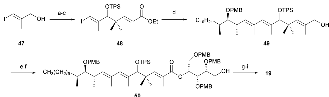
Scheme 7 Synthesis of 19. Reagents and conditions: (a) i) \text{MnO}_2 , \text{CH}_2\text{Cl}_2 , ii) methyl isobutyrate, LDA, THF, -78^{\circ}\text{C} , 2 steps, 80%; (b) i) TPSCl, imidazole, DMF, ii) DIBAL, \text{CH}_2\text{Cl}_2 , -78^{\circ}\text{C} , 2 steps, 97%; (c) i) (\text{COCl})_2 , DMSO, \text{Et}_3\text{N} , \text{CH}_2\text{Cl}_2 , ii) \text{PPh}_3=\text{C}(\text{CH}_3)\text{CO}_2\text{Et} , toluene, reflux, 2 steps, 91%; (d) i) 3, 9-BBN, THF, rt then \text{PdCl}_2(\text{dppf}) , \text{K}_3\text{PO}_4 , DMF, \text{H}_2\text{O} , 65^{\circ}\text{C} , ii) DIBAL, \text{CH}_2\text{Cl}_2 , -78^{\circ}\text{C} , 2 steps, 86%; (e) i) (\text{COCl})_2 , DMSO, \text{Et}_3\text{N} , \text{CH}_2\text{Cl}_2 , ii) \text{NaClO}_2 , \text{NaH}_2\text{PO}_4 , t\text{-BuOH} , \text{H}_2\text{O} , 2 steps, 86%; (f) i) 5, EDCI·HCl, DMAP, \text{CH}_2\text{Cl}_2 , reflux, ii) HCl, THF, 2 steps, 65%; (g) TBAF, AcOH, THF, 50^{\circ}\text{C} , 89%; (h) i) Dess–Martin periodinane, pyridine, \text{CH}_2\text{Cl}_2 , ii) \text{NaClO}_2 , \text{NaH}_2\text{PO}_4 , t\text{-BuOH} , \text{H}_2\text{O} , 2 steps, 41%; (i) \text{BCl}_3 , \text{CH}_2\text{Cl}_2 , -78^{\circ}\text{C} , 50%.
