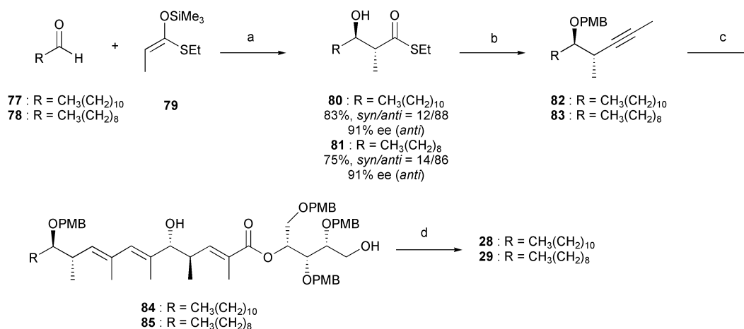
Scheme 13 Synthesis of 28 and 29 . Reagents and conditions: (a) ( S )-3,3,6,6- \text{I}_4\text{BINOL} , \text{Zr}(\text{O}t\text{-Bu})_4 , \text{PrOH} , \text{H}_2\text{O} , toluene, 0^\circ\text{C} ; (b) i) \text{LiAlH}_4 , THF, ii) \text{PMPCH}(\text{OMe})_2 , p\text{-TsOH} , \text{CH}_2\text{Cl}_2 , iii) DIBAL, \text{CH}_2\text{Cl}_2 , 0^\circ\text{C} , iv) (\text{COCl})_2 , DMSO, \text{Et}_3\text{N} , \text{CH}_2\text{Cl}_2 , v) \text{CBr}_4 , \text{PPh}_3 , \text{CH}_2\text{Cl}_2 , 0^\circ\text{C} , vi) n\text{-BuLi} , \text{MeI} , THF, 6 steps, 41% ( 82 ), 86% ( 83 ); (c) i) 13 , 9-BBN, THF, then \text{PdCl}_2(\text{dppf}) , \text{K}_3\text{PO}_4 , DMF, \text{H}_2\text{O} , 65^\circ\text{C} , ii) \text{HCl} , THF, 2 steps, 53% ( 84 ), 58% ( 85 ); (d) i) Dess–Martin periodinane, pyridine, \text{CH}_2\text{Cl}_2 , ii) \text{NaClO}_2 , \text{NaH}_2\text{PO}_4 , t\text{-BuOH} , \text{H}_2\text{O} , iii) \text{BCl}_3 , \text{CH}_2\text{Cl}_2 , -78^\circ\text{C} .
