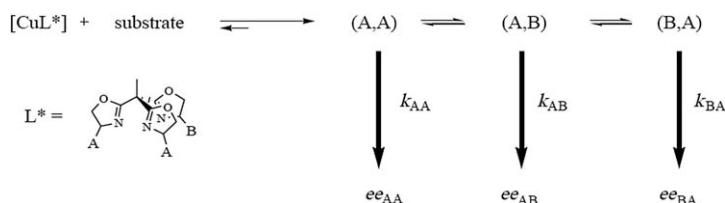
Scheme 5.
