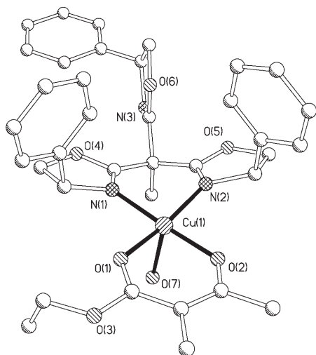
Figure 2. Molecular structure of the copper complex [\text{Cu}^{\text{II}}(\text{Ph}_3\text{-triso}(R,S,S))(\kappa^2\text{-}O,O'\text{-MeCOCHCOOEt})(\text{H}_2\text{O})]^+[\text{ClO}_4]^- ( 2 ). The counterion is omitted for clarity. The principal bond lengths and angles are given in Table 2. Hydrogen atoms omitted for clarity.
