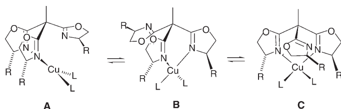
Scheme 1. Equilibrium between the three symmetry-equivalent triso isomers with the bicoordinate stereodirecting ligand.
