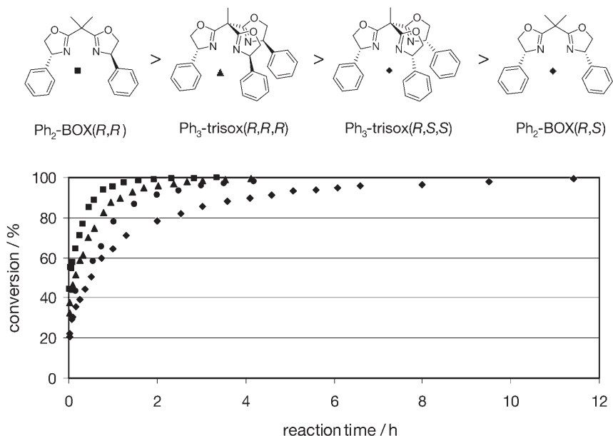
Figure 3. Conversion curves of the Cu-catalysed C–N coupling reaction (1.0 mol% catalyst loading) for the four catalysts bearing \text{Ph}_3\text{-triso}(R,R,R) , \text{Ph}_3\text{-triso}(R,S,S) as well as \text{Ph}_2\text{-BOX}(R,R) and \text{Ph}_2\text{-BOX}(R,S) as stereodirecting ligands.
