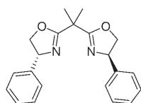
Ph 2 -BOX( R,R ) ( C 2 )
