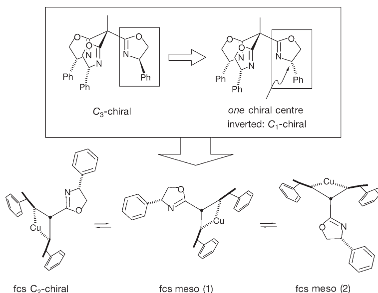
Scheme 4. Effect of the inversion of a chiral centre in Ph_3 -trisox (top) leading to an equilibrium between three inequivalent dicoordinate species in solution (bottom). In two of these the arrangement of the oxazoline substituents at the rings coordinated to the metal centre correspond to a local meso -environment.
