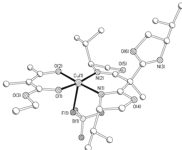
Figure 1. Molecular structure of the copper complex [Cu^{II}(iPr_3\text{-trisox})(\kappa^2\text{-}O,O'\text{-MeCOCHCOOEt})]^+ [BF_4]^- ( 1 ). The principal bond lengths and angles are given in Table 2. Hydrogen atoms omitted for clarity.
