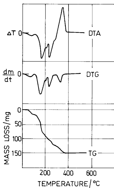
Fig. 3. TG, DTG and DTA curves for the reaction of ammonium fluoride with yttrium oxide (NH 4 F:Y 2 O 3 = 9:1).
