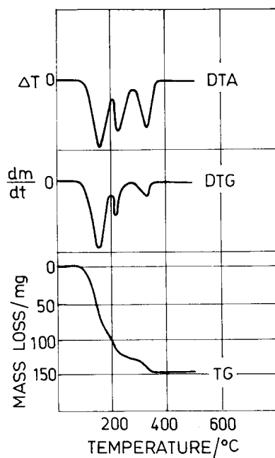
Fig. 2. TG, DTG and DTA curves for the reaction of ammonium fluoride with yttrium oxide (NH 4 F:Y 2 O 3 = 6:1).
