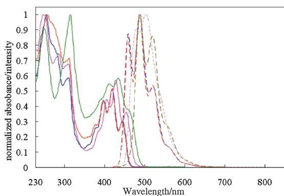
Figure 3. UV-vis (solid lines) and fluorescence spectra (dashed line) of H 2 QQs 2c–2f in CH 2 Cl 2 ( 2c : blue; 2d : red; 2e : pink; 2f : green).
