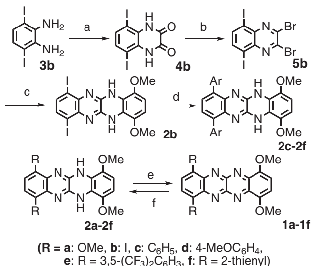
Scheme 1. Reagents and conditions: (a) (COOEt) 2 , NaOEt, benzene, reflux; (b) PBr 3 , reflux; (c) 3,6-dimethoxy-1,2-phenylenediamine ( 3a ), EtOH, reflux; (d) arylboronic acid, [Pd(PPh 3 ) 4 ], K 2 CO 3 , H 2 O–THF, reflux; (e) DDQ, CHCl 3 ; (f) Na 2 S 2 O 4 , THF–H 2 O.
