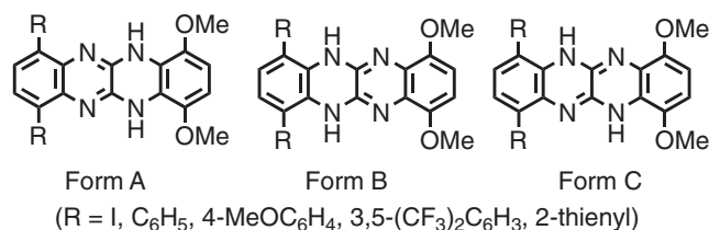
Scheme 2. Possible isomers of H 2 QQs 2b–2f .
