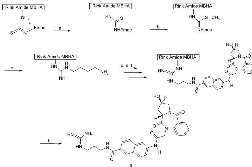
Scheme 3. Synthesis of 3 a
