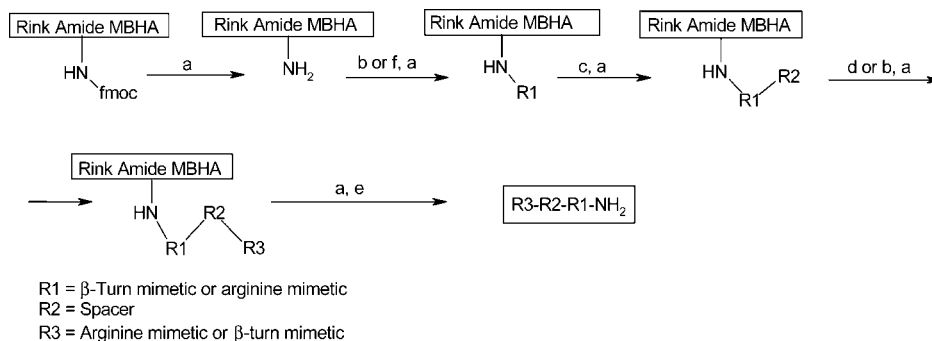
Scheme 1. General Scheme of Parallel SPPS a
