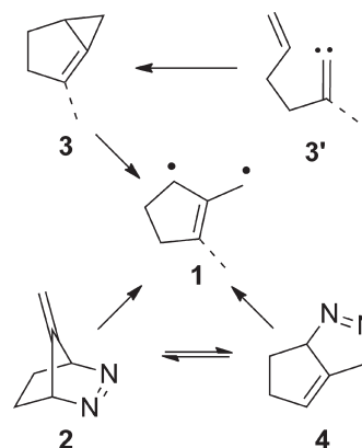
Scheme 1. Generation of Methylcyclopentene TMM Diyl 1
