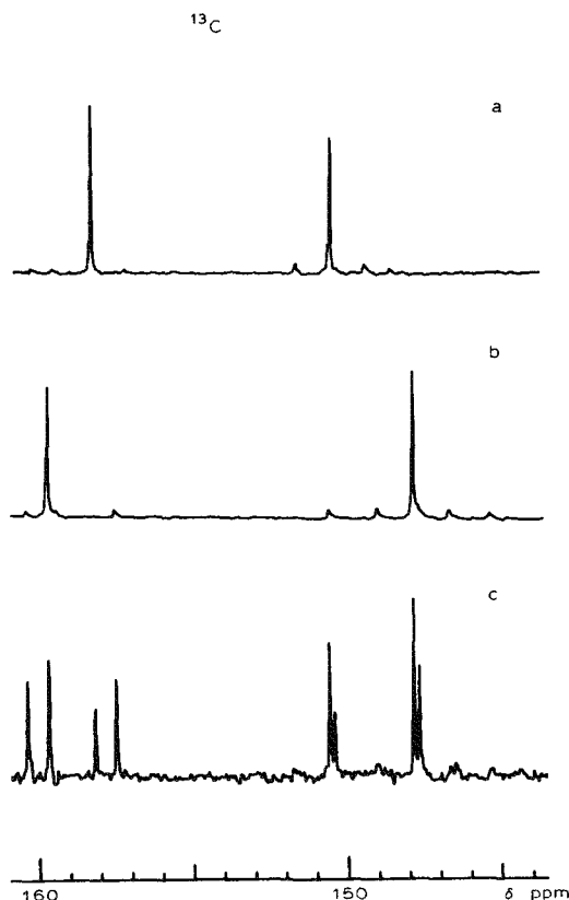
Fig. 1. Carbon-13 NMR spectra of the vinyl region of related divinylmercury compounds: (a) di[( E )-1-deceny]mercury ( \delta 158.3 and 150.2 ppm); (b) bis[( E )-5-chloro-1-phenenyl]mercury ( \delta 159.7 and 147.8 ppm); (c) reaction products obtained via addition of ( E )-5-chloro-1-pentenylboronic acid to ( E )-1-deceny]mercuric acetate ( \delta 160.4, 159.7, 158.3, 157.5, 150.5, 150.2, 147.8, and 147.6 ppm) which corresponds to the unsymmetrical divinylmercury reagent and the two symmetrical, divinylmercury equilibration products.
