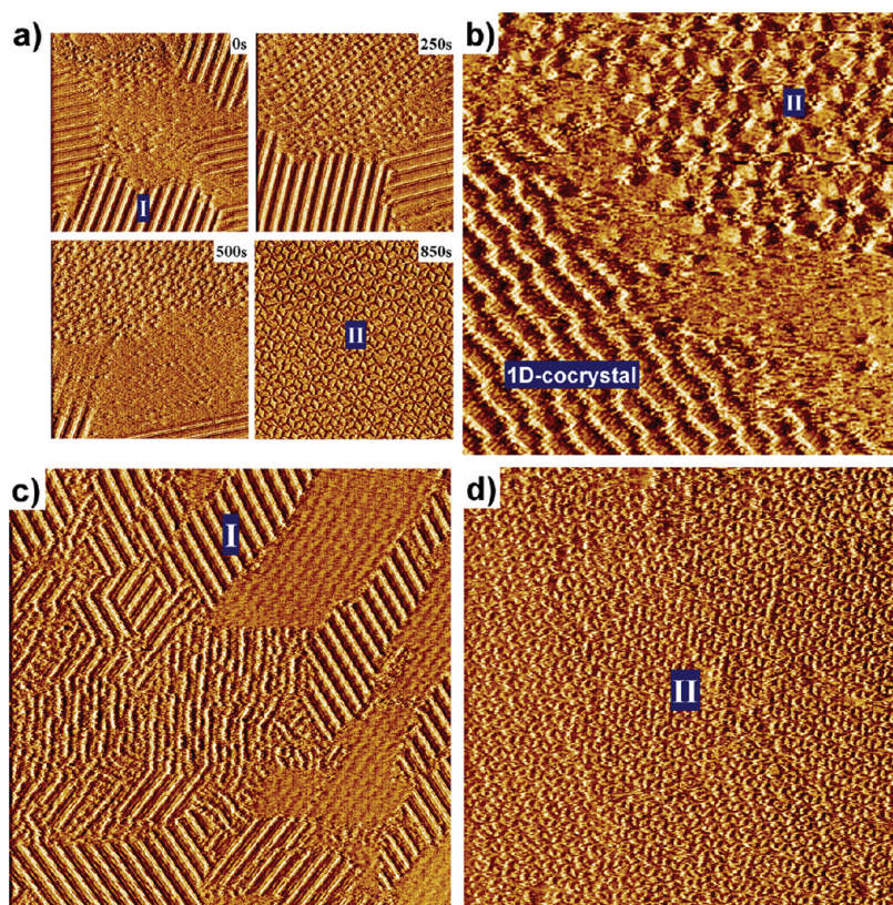
Figure 2. Assemblies obtained from the competition study of 18-amide and 17- m -diester . Blue insets identify phases. (a) STM images ( 100 \times 100 \text{ nm}^2 ) showing phase transformation from the close packed phase (phase I) to the rhombic nanoporous network (phase II) observed at 1:6 ( 18-amide / 17- m -diester ). (b) STM image ( 50 \times 50 \text{ nm}^2 ) showing coadsorption of phase II of 18-amide and 1D-cocrystal at a 1:11 ratio. (c) STM image ( 200 \times 200 \text{ nm}^2 ) obtained from 1:9 ratio with 52 \mu\text{M} 18-amide . (d) STM image ( 200 \times 200 \text{ nm}^2 ) obtained from 1:9 ratio with 10 \mu\text{M} 18-amide .
