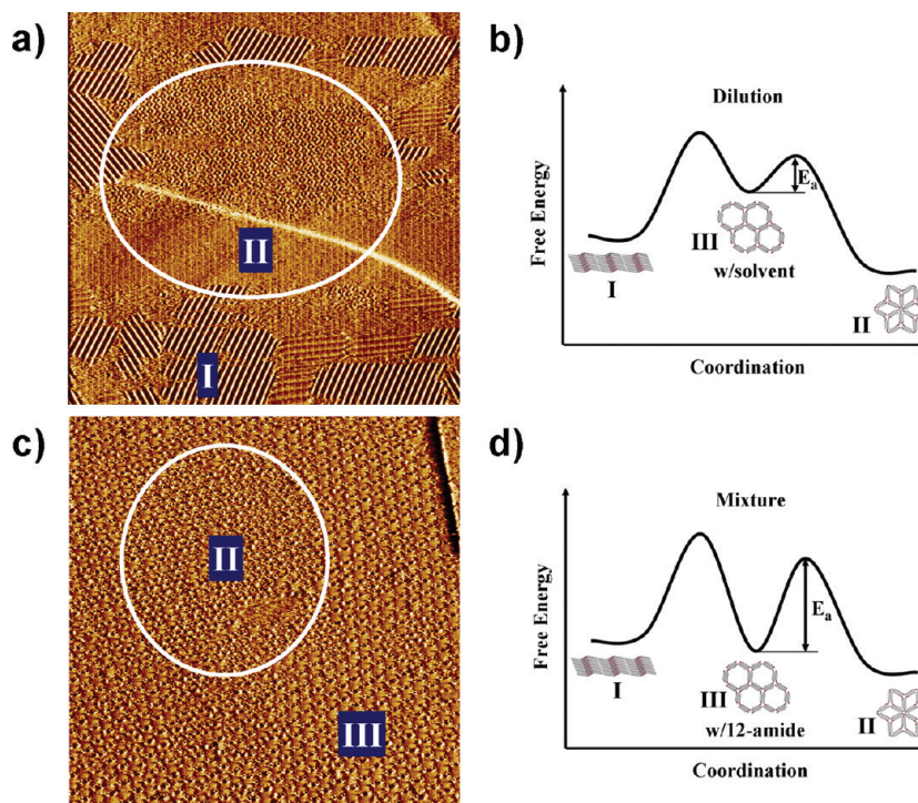
Figure 6. STM images ((a) 400 × 400 nm 2 , (c) 200 × 200 nm 2 ) and reaction coordinate diagram of the phase transformation from (a, b) the homogeneous solution of 25 μM and (c, d) the mixture of 1:3 (18-amide/12-amide) with 25 μM of 18-amide. In the 18-amide homogeneous solutions, phase III is observed as a kinetic intermediate at the boundary area between phase I and II. However, in the mixture with 12-amide, phase III is observed as a major phase and slowly transformed to phase II where phase I was rarely observed, indicating that phase III can be more stable than phase I in the mixture.
