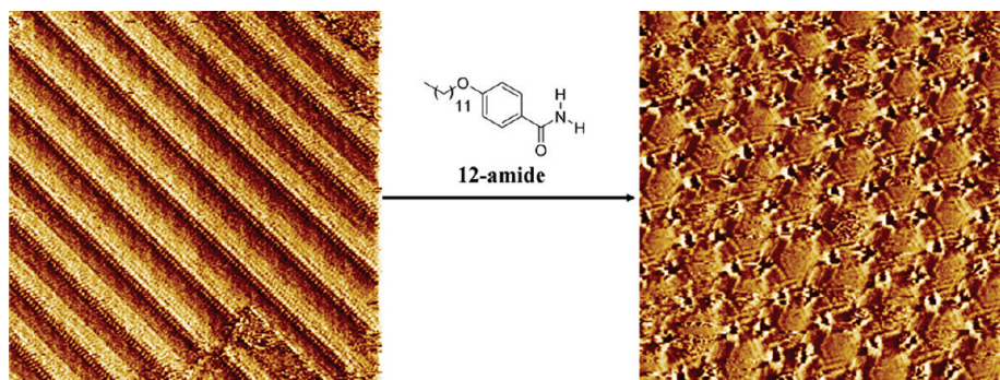
Figure 7. STM images (50 × 50 nm 2 ) showing the role of 12-amide molecules as stabilizers of phase III. Phase I formed from the homogeneous solution was transformed to phase III by adding 12-amide solution to make a 1:3 mixture (18-amide/12-amide).
