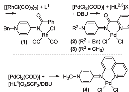
Scheme 3. Syntheses of Complexes 1–4
