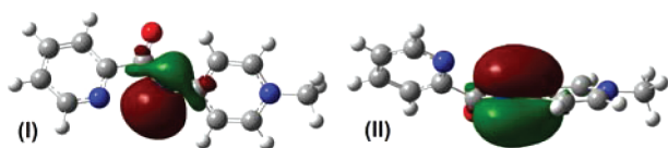
Figure 1. Frontier NBO orbitals: (I) lone pair on N2 and (II) the \pi bond between N2 and C7 in \text{L}^3 .
