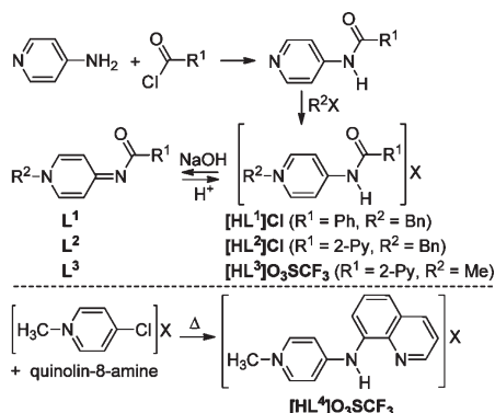
Scheme 2. Syntheses of Alkylpyridinium Carboxamides [\text{HL}^{1-3}]\text{X} , PYA Ligands \text{L}^{1-3} , and Methylpyridinium Amine [\text{HL}^4]\text{X}
