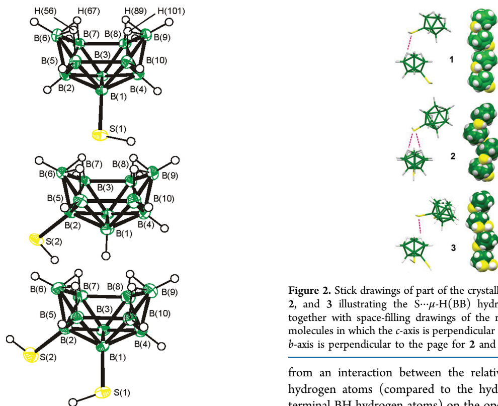
Figure 1. Crystallographically determined molecular structures of [1-(HS)- nido - \text{B}_{10}\text{H}_{13} ] 1 (top), [2-(HS)- nido - \text{B}_{10}\text{H}_{13} ] 2 (center), and [1,2-(HS) _2 - nido - \text{B}_{10}\text{H}_{12} ] 3 (bottom), with 50% probability ellipsoids for the non-hydrogen atoms. Listings of geometric parameters are given in the Supporting Information.
