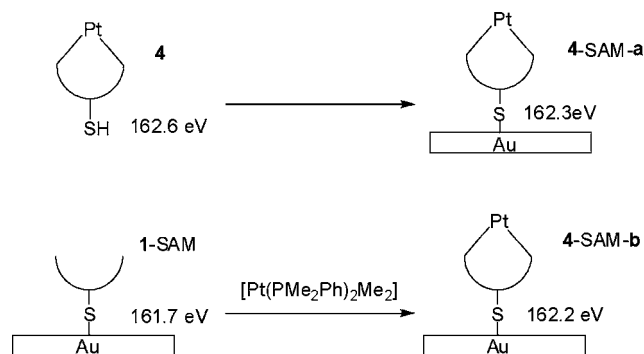
Scheme 4. Reaction Scheme for the Preparation of 4 -SAM-a and 4 -SAM-b, Showing Also the Binding Energies of the Sulfur 2p Electrons
