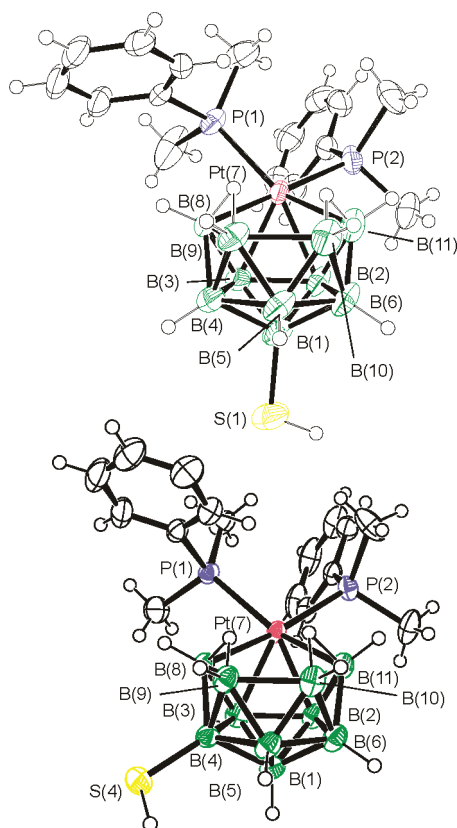
Figure 3. Crystallographically determined molecular structures of [1-(\text{HS})\text{-}7,7\text{-(PMe}_2\text{Ph)}_2\text{-nido-}7\text{-PtB}_{10}\text{H}_{11}] 4 (upper) and [4-(\text{HS})\text{-}7,7\text{-(PMe}_2\text{Ph)}_2\text{-nido-}7\text{-PtB}_{10}\text{H}_{11}] 5 (lower) with 50% probability ellipsoids for the non-hydrogen atoms. A \text{CH}_2\text{Cl}_2 solvent molecule in 5 is not shown. Listings of geometric parameters are given in the Supporting Information.
