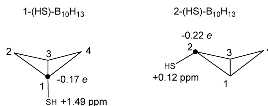
Scheme 2. Calculated Atomic Charges on the Boron Atom Vertices B(1) in [1-(\text{HS})\text{-B}_{10}\text{H}_{13}] and B(2) in [2-(\text{HS})\text{-B}_{10}\text{H}_{13}] , Together with the Measured Thiol Proton NMR Chemical Shifts
