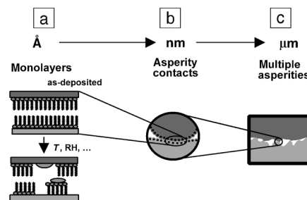
Figure 2. Length scales that must be linked to understand micromachine device performance include (a) as-deposited and potentially degraded coatings (angstrom scale), (b) local adhesion measurement (nanometer scale), and (c) asperity interaction influencing micromachine deflections (micrometer scale).
