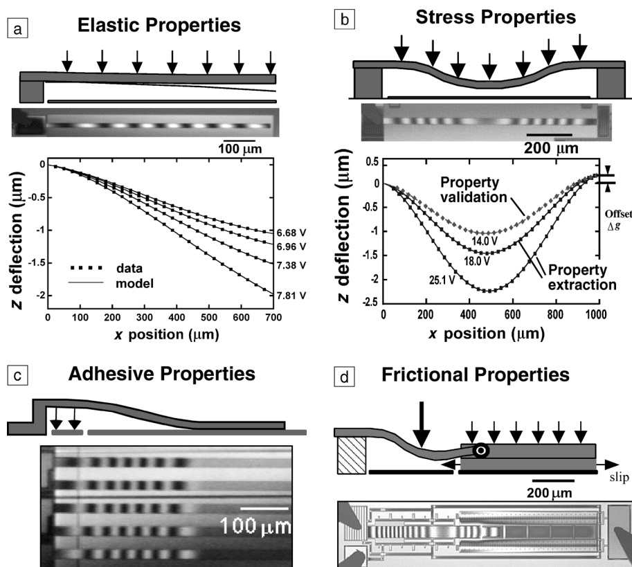
Figure 1. Microtribology laboratory on a chip. Integrated interferometry and finite element modeling in concert with optimized test structure design are used to determine thin-film and interfacial properties. See text for description of (a)–(d).
