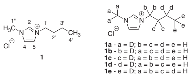
Figure 1. Structure and numbering of [C_4mim]Cl ( 1 ) and its deuterium isotopologues ( 1a–e ).
