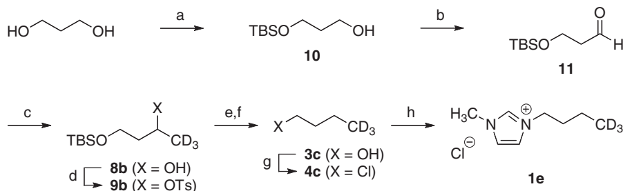
Scheme 4. (a) TBDMS-Cl, NaH, THF (96%); (b) (COCl) 2 , DMSO, Et 3 N, CH 2 Cl 2 ; (c) CD 3 I, Mg, Et 2 O (65% over both steps); (d) TsCl, pyridine, CH 2 Cl 2 (94%); (e) LiAlH 4 , Et 2 O; (f) HCl/H 2 O (60% over both steps); (g) SOCl 2 (74%); and (h) 1-methylimidazole (quantitative).
