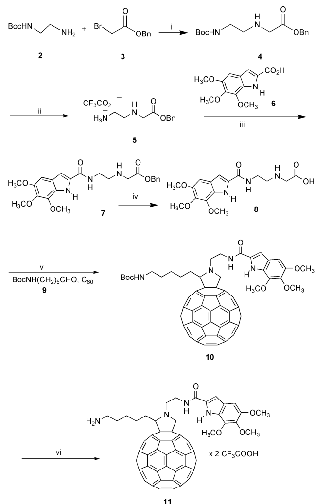
Scheme 1 Reagents: i, dioxane, 0 °C, then rt 18 h; ii, TFA, CH 2 Cl 2 , rt, 20 min; iii, NMM, HOBT, EDC, CH 2 Cl 2 ; iv, Pd/C 10%, H 2 , MeOH; v, toluene, reflux, 50 min; vi, TFA, CH 2 Cl 2 , rt, 1 h.
