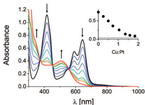
Figure 6. UV–vis absorption of 1.96 \times 10^{-4} M solutions of 2 in benzene containing 0–1.83 equiv of CuOTf. The black spectrum corresponds to pure 2 and the red one to 2 in the presence of a large excess of CuOTf. (Inset) Absorbance at 644 nm as a function of the Cu:Pt ratio. The dashed line corresponds to the absorbance in the presence of excess CuOTf.
