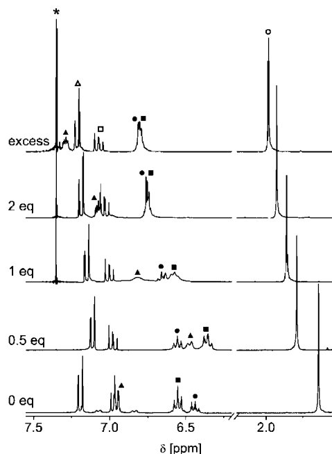
Figure 11. ^1\text{H} NMR spectra of \sim 25 mM solutions of 3 in \text{CD}_2\text{Cl}_2 containing various amounts of CuOTf. Peak assignment: \text{PtPh}^{2,6} , \Delta ; \text{PtPh}^{3,5} , \blacksquare ; \text{PtPh}^4 , \bullet ; \text{NAr}^{3,5} , \blacktriangle ; \text{NAr}^4 , \square ; CMe, \circ . The peak of benzene coming from \text{CuOTf} \cdot 1/2\text{C}_6\text{H}_6 is marked with *. It is absent in the spectrum with 0.5 equiv of CuOTf because the latter was recorded from crystallized 6a .
