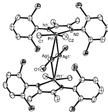
Figure 2. ORTEP representation of the X-ray crystal structure of 5b . Ellipsoids are drawn at 50% probability. For clarity, only the silver-bound oxygen atom of the CF 3 SO 3 − units is plotted, and an unbound benzene molecule is omitted. Selected distances [Å], angles [deg], and torsion angles [deg]: Ag1–Ag1' 2.6972(2), Ag1–O1 2.354(3), Ag1–Pt1 2.8290(6), Ag1–Pt1 2.9097(5), Pt1–C1 2.039(4), Pt1–C2 2.043(4), Pt1–N1 2.117(3), Pt1–N2 2.118(3), Ag1'–Ag1–Pt1 63.489(15), Ag1–Pt1–Ag1' 56.047(15), O1–Ag1'–Ag1 164.82(8), C1–Pt1–C2 89.28(17), C1–Pt1–N1 97.19(14), C2–Pt1–N2 96.28(14), N1–Pt1–N2 75.59(11), Pt1–Ag1–Ag1'–Pt1' 180.0.
