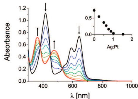
Figure 7. UV–vis absorption of 1.97 \times 10^{-4} M solutions of 2 in benzene containing 0 (black) to 1.53 (red) equiv of AgOTf. (Inset) Absorbance at 644 nm as a function of the Ag:Pt ratio.
