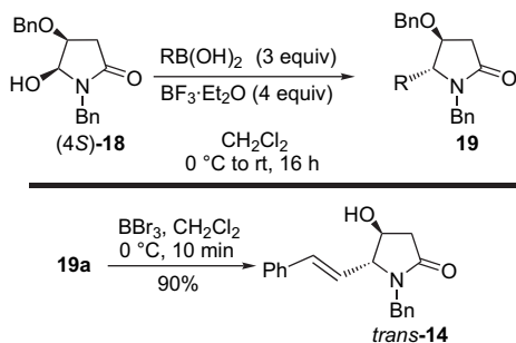
Scheme 6.
