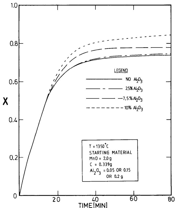
Fig. 7. The effect of additions of \text{Al}_2\text{O}_3 on the reduction of \text{MnO} by graphite.
