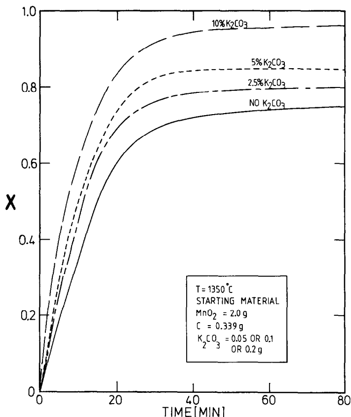
Fig. 4. The effect of additions of \text{K}_2\text{CO}_3 on the reduction by graphite.
