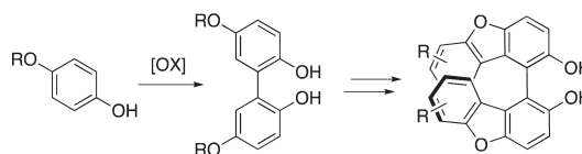
Scheme 4. Alternative Approach to Bis-dibenzofuranol Derivatives
