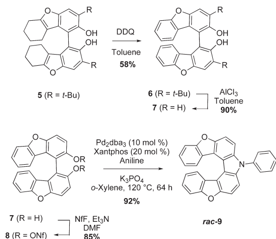
Scheme 2. Synthesis of Dioxaza[7]helicene 9
