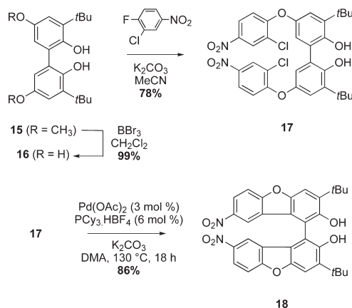
Scheme 5. Synthesis of Substituted Bis-dibenzofuran 18
