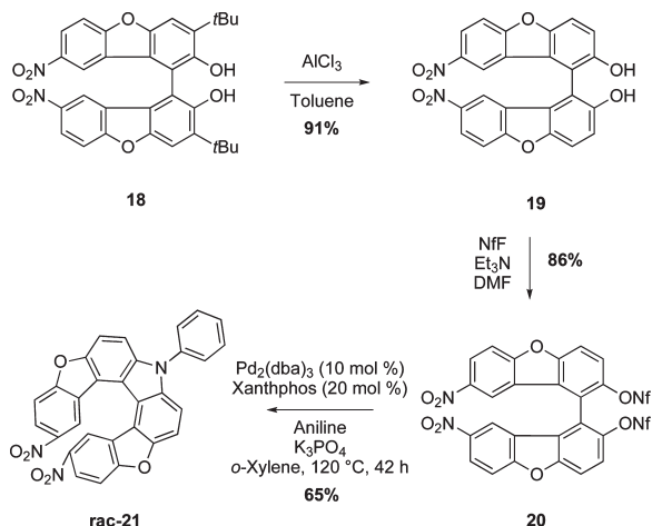
Scheme 6. Synthesis of 2,13-Dinitrodioxa-aza[7]helicene 21
