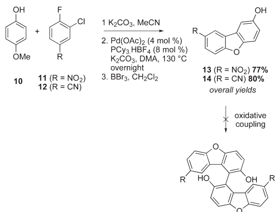
Scheme 3. Synthesis and Oxidative Coupling of Substituted Dibenzofuran Moieties
