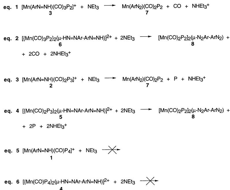
Scheme 3. P = P(OMe) 3 ( a ), P(OEt) 3 ( b ) or P(OPh) 3 ( c ); Ar = C 6 H 5 ; Ar–Ar = 4,4′-C 6 H 4 –C 6 H 4 .
