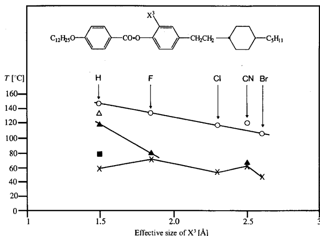
Fig. 3. Transition temperatures vs. the size of the lateral substituent \text{X}^3 (X: crystal-smectic 3/smectic C/nematic transition; ■: smectic 3-smectic C transition; ▲: smectic C-smectic A/nematic transition; △: smectic A-nematic transition; ○: nematic-isotropic transition)
