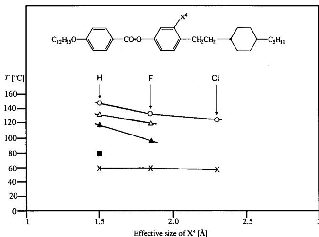
Fig. 4. Transition temperatures vs. the size of the lateral substituent \text{X}^4 (X: crystal-smectic 3/smectic C/nematic transition; ■: smectic 3-smectic C transition; ▲: smectic C-smectic A transition; △: smectic A-nematic transition; ○: nematic-isotropic transition)
