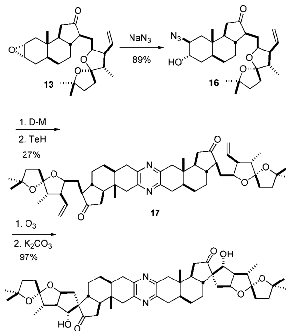
Bis-18, 18'-Desmethyl Ritterazine N 4
