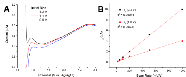
Figure 4: (A) Cathodic scans after activating the hematite substrate at the indicated bias under white light illumination. Peaks appear as surface species are being reduced. (B) Peak current exhibits a linear dependence on scan rate, confirming this is a surface process.
