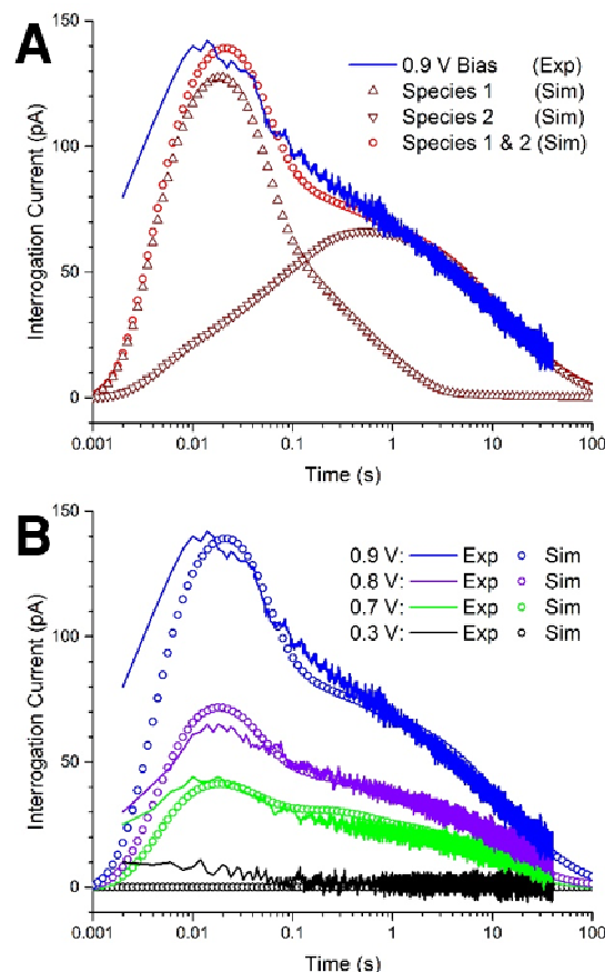
Figure 5: (A) Experimental interrogation current collected after a bias of 0.9 V (blue line). Best fits modeled with a single fast reacting species (up triangles), with a single slow reacting species (down triangle), and a linear combination of the two (red circles), are overlaid. (B) Best fits to experimental data using the two species model for a range of activating potentials. Satisfactory fitting of experimental data is achieved over several orders of magnitude in time. Interrogations were performed with a 4 \mu\text{m} carbon disk electrode in an aqueous solution of 50 \mu\text{M} ferricyanide in 100 mM borate buffer (pH=9.3) under broadband illumination.
