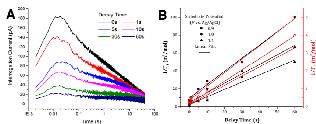
Figure 7: (A) Surface interrogations recorded after a delay that followed substrate activation at 0.9 V vs Ag/AgCl for 40 s show a decreasing interrogation current as the delay increases. (B) Coverages of species 1 and 2 as a function of delay time fit to second order kinetics. The plotted fits give the disproportionation kinetics as k_{d1} = 1.2 \times 10^5 \pm 0.2 \times 10^5 and k_{d2} = 6.3 \times 10^3 \pm 0.9 \times 10^3 \text{ m}^2/(\text{mol} \cdot \text{s}) .
