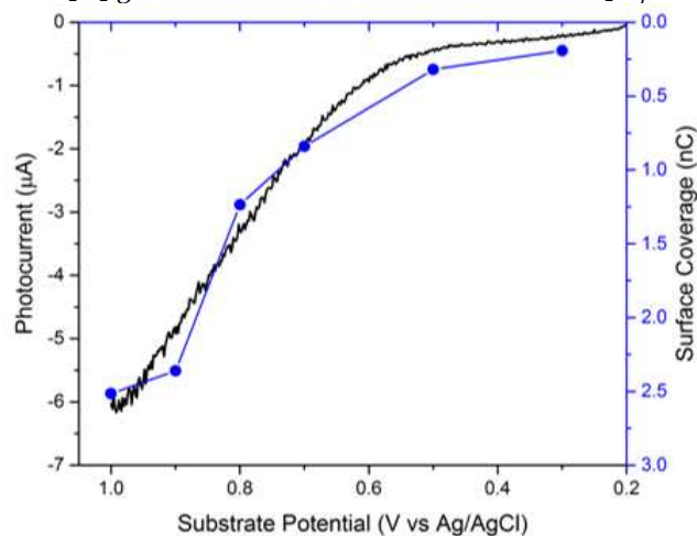
Figure 6: Total charge collected by SI-SECM (blue circles) overlaid on a I(V) curve of Hematite (black line).
