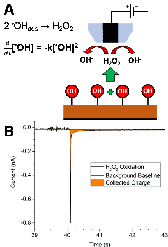
Figure 8: (A) Schematic of the tip collection step of transient hydrogen peroxide collection experiments. (B) Tip current as a function of time during a transient substrate generation tip collection experiment. In this setup, a 12.5 \mu\text{m} tip electrode is positioned 10 \mu\text{m} from the surface and biased at 0.40 V for the duration of the experiment. The substrate is activated to perform steady state water oxidation for the first 40 seconds. Substrate illumination and bias are removed after 40 seconds while continuing to record tip current.
