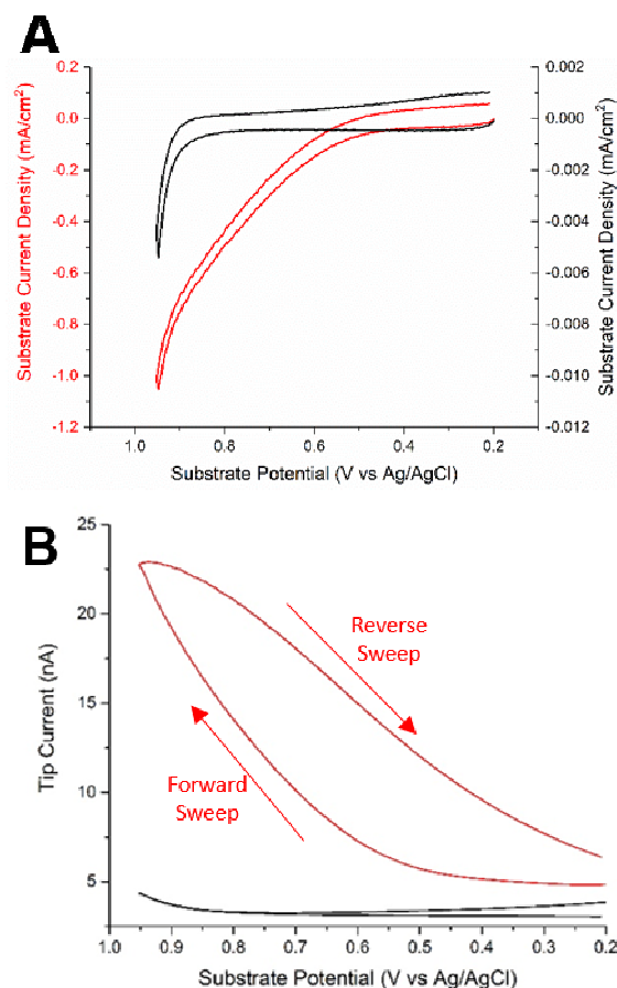
Figure 3: (A) Cyclic voltammograms of a \text{Ti-Fe}_2\text{O}_3 electrode in the dark (black curve) and under broadband illumination (red curve) recorded in 0.1 M NaOH. (B) Current recorded by a 12.5 \mu\text{m} radius Pt electrode positioned close to the surface and biased at -0.4 V to reduce oxygen during the substrate CVs shown in A.
